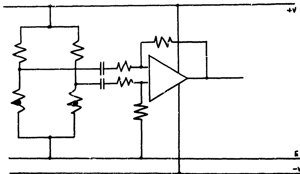
Fig 6 Circuit schematic
