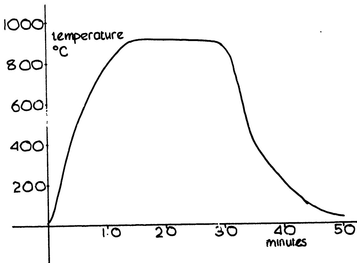
Fig 4 Firing profile
