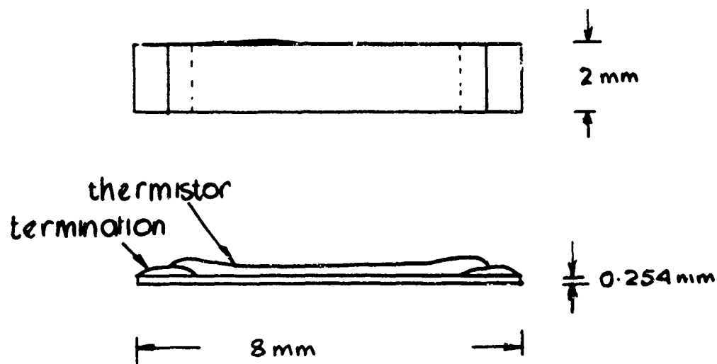
Fig 5 Thick film thermistor sensor
