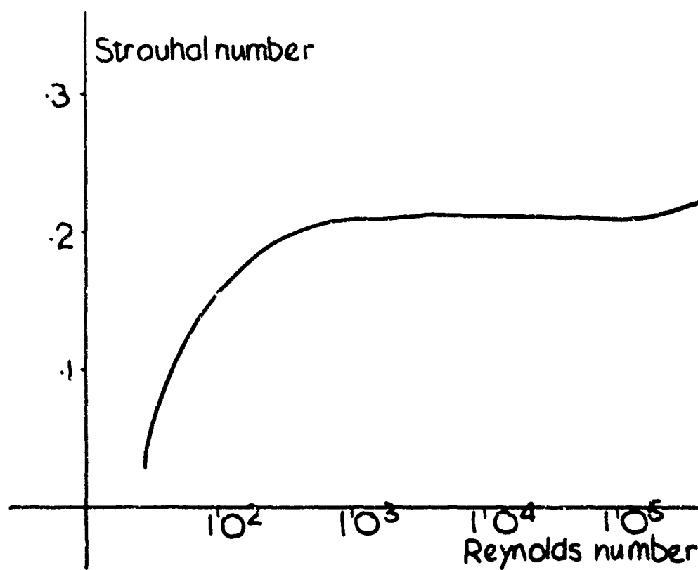
Fig 2 Strouhal number
