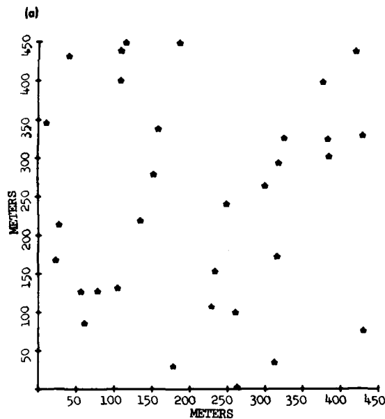
FIG. 5. Random array of 32 elements (a) y versus x , (b) z versus x , (c) z versus y .
