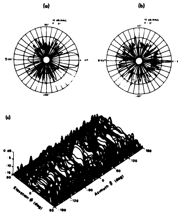
FIG. 6. Random array beam patterns ( B_m: \theta = \phi = 0^\circ ).
