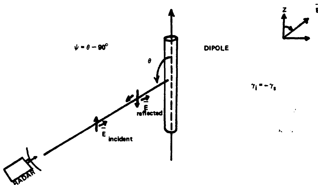
Figure 3. Scattering geometry for a full wave dipole.
