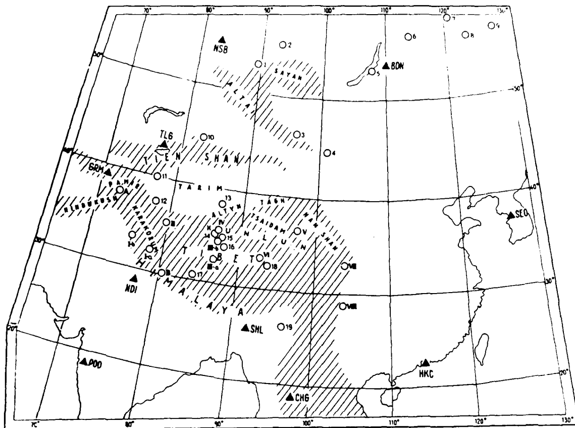
Map of Asia showing stations used; epicenters of earthquakes for which seismograms are shown in Figures 2 (Arabic numerals), 3 (Roman numerals), and 4 (A and B); and areas of high mountains (hatched regions).
