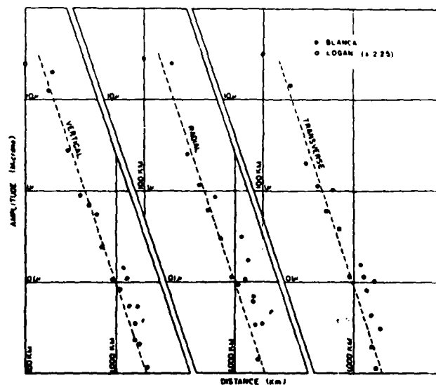
Amplitudes of 3.5-km/sec shear waves from a 19-kt underground explosion. Curves are drawn proportional to the inverse cube of the distance.
