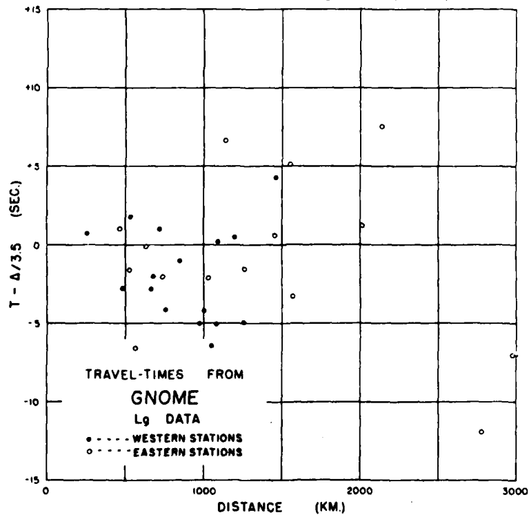
Travel time residuals for L_g waves relative to constant velocities for eastern and western stations.
