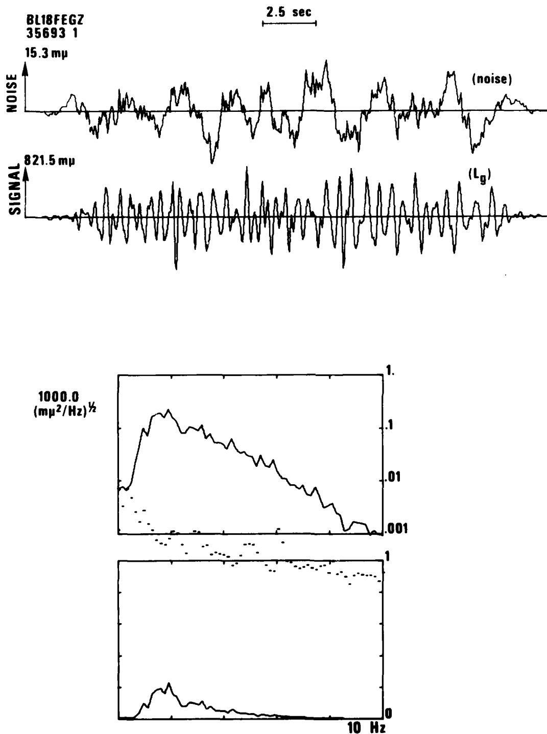
Figure 38. 18 February L g wave signals and noise, waveforms and spectra at BLWV.
