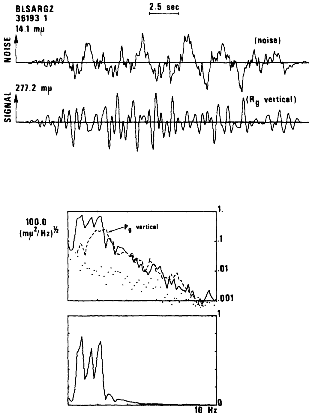
Figure 29a. SALMON L g waves and noise, signal and spectra at BLWV, vertical component.
