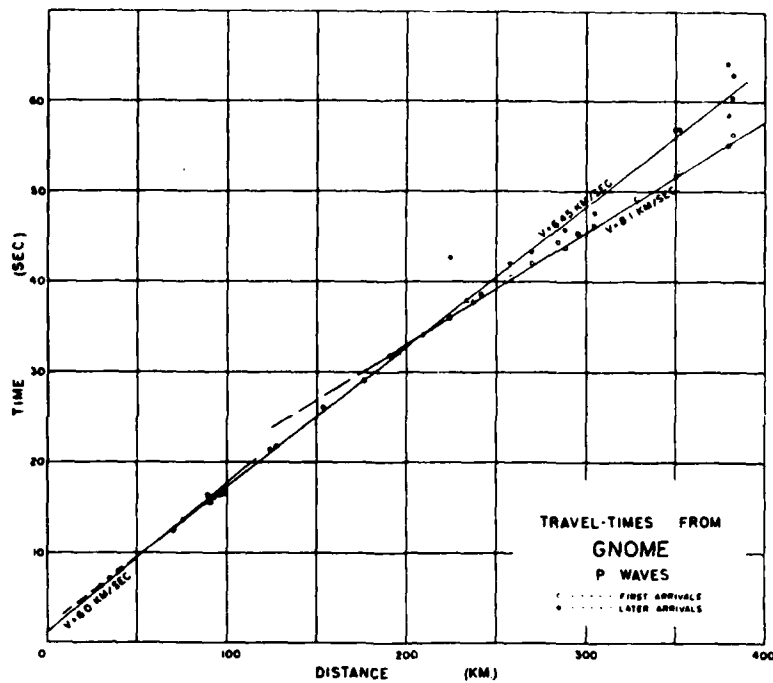
Travel times from GNOME for close range stations (P waves).
