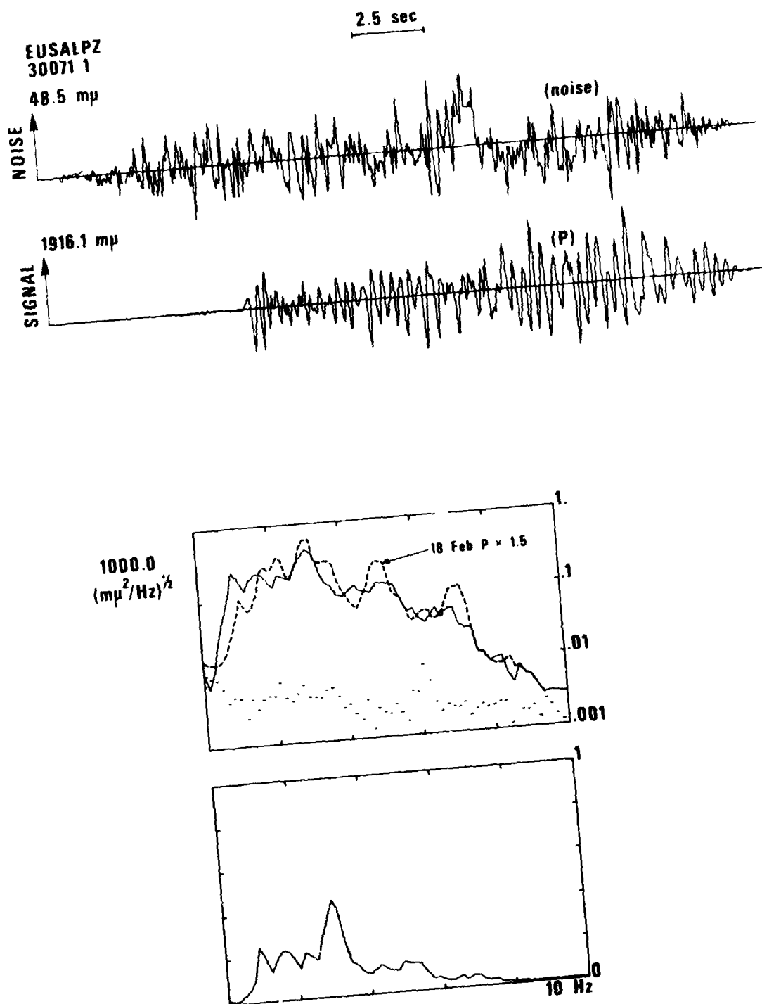
Figure 31. SALMON P waves and noise, signal and spectral at EUAL a distance of 242 km. Note overlay of 18 February 1964 earthquake at EUAL.
