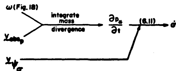
Fig. 19. Flow chart depicting the calculation of \sigma .
