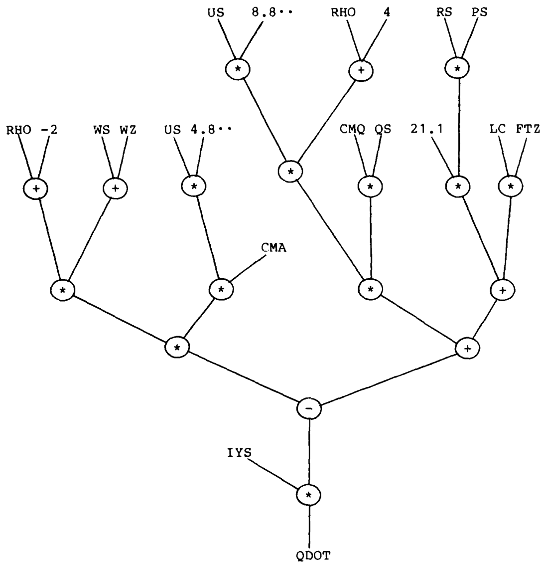
Figure 8 - Parse Tree of Expression for QDOT
