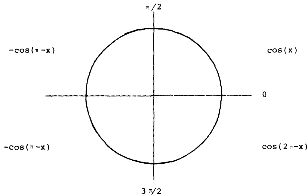
Figure 5 - Cosine Function Relationships
