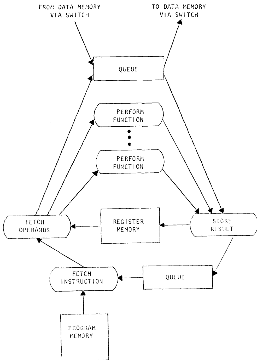
Figure 1 - Processor Organization
