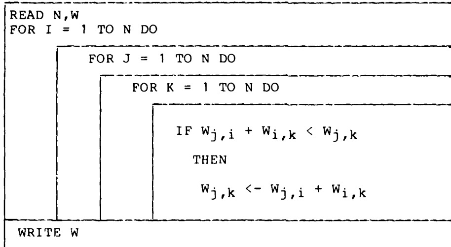
Figure 20 - Minimum Path Algorithm
