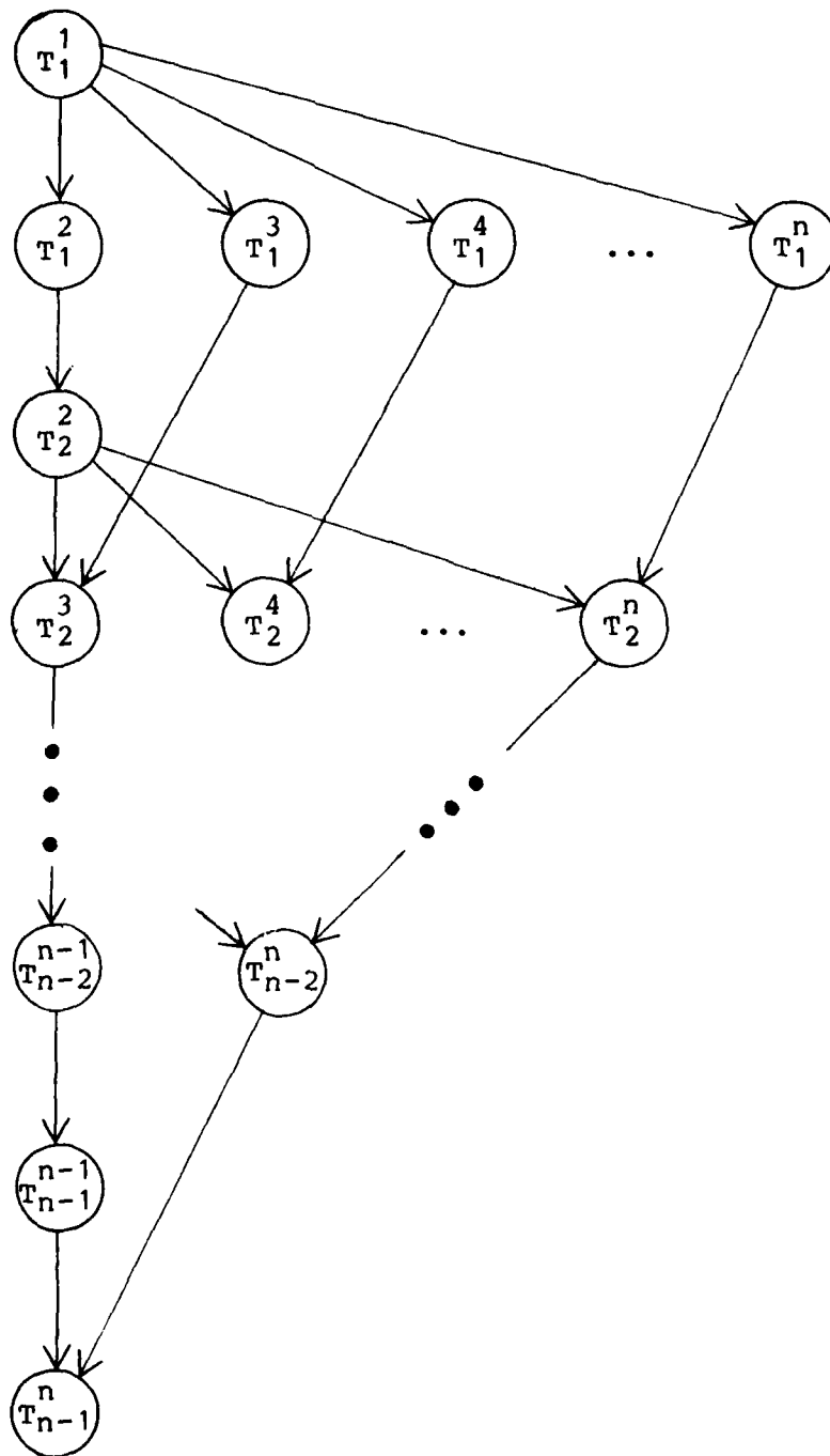
Figure 24 - Maximally Parallel Task System Equivalent to C
