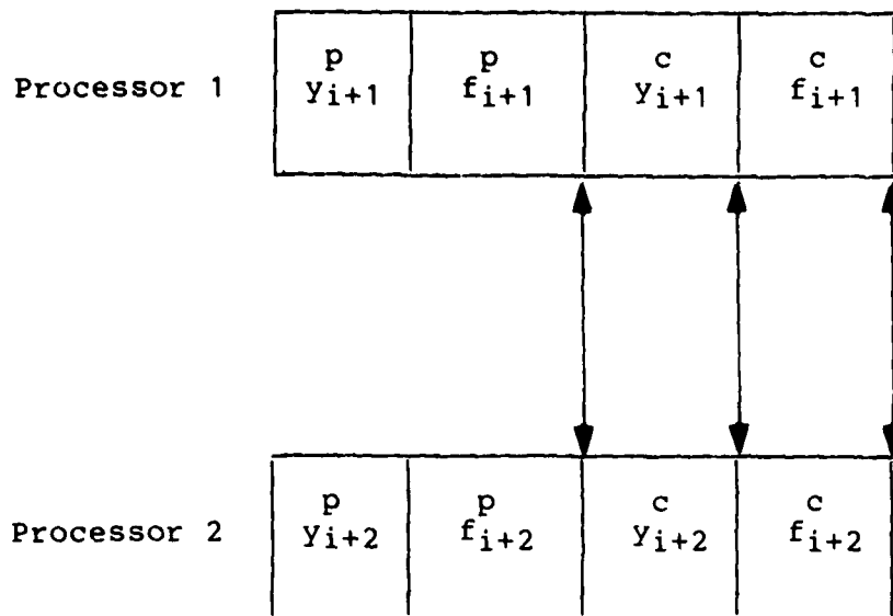
Figure 19 - Parallel Scheme for BPC
