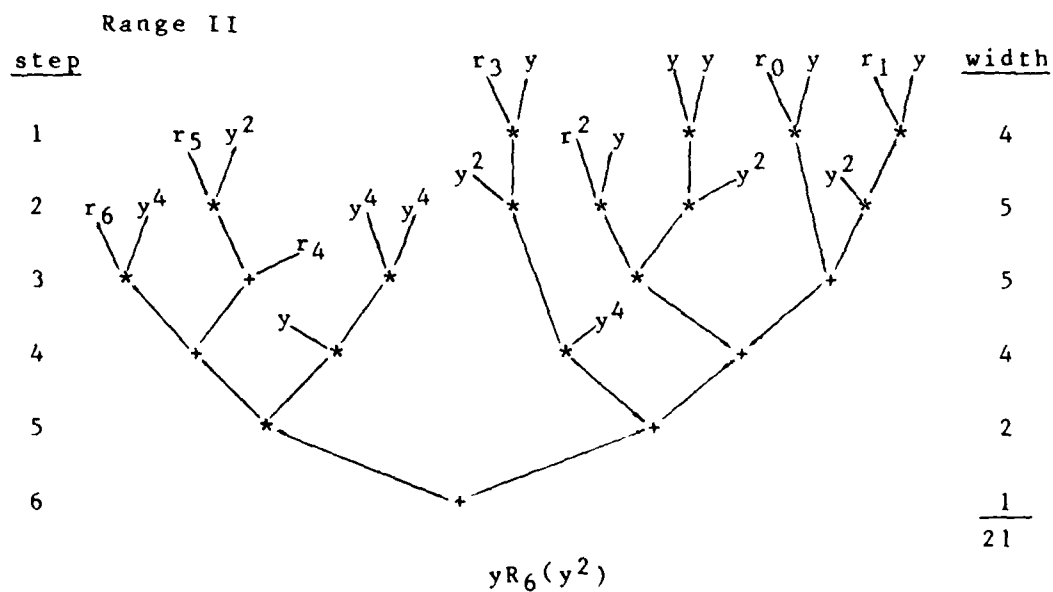
Figure 7 - Logarithm Task 7 Computational Trees
