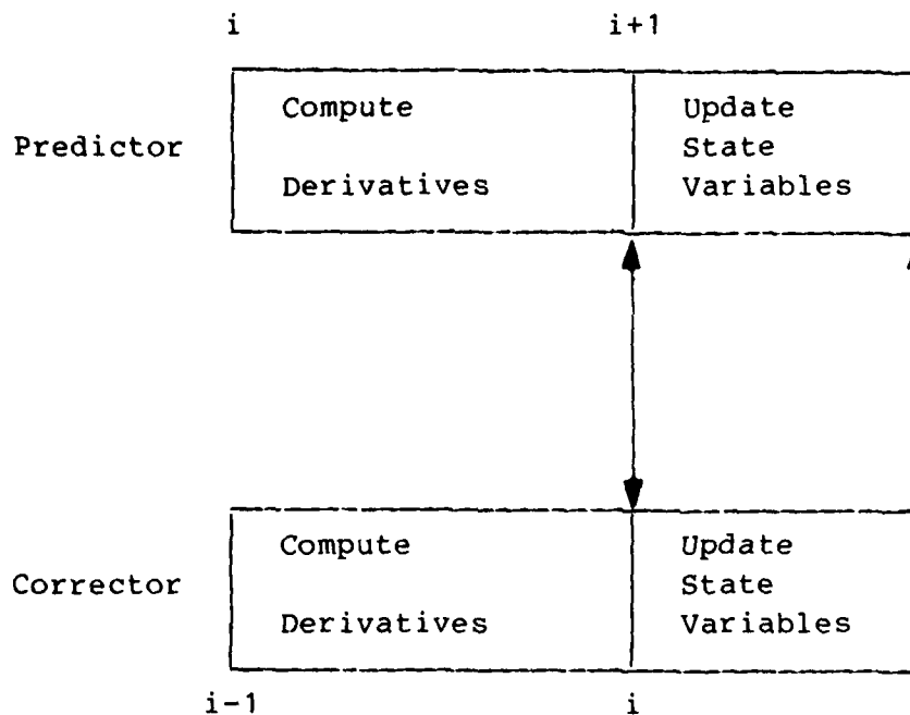
Figure 18 - Parallel PC Scheme
