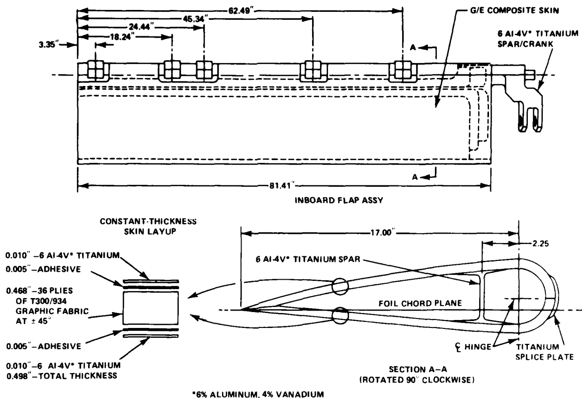
Figure 2 - Composite Foil Flap Component
