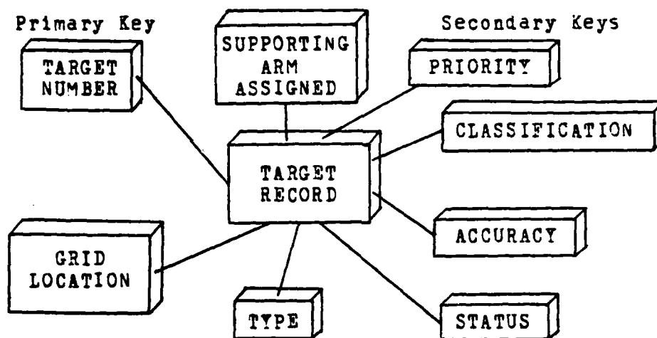
Figure 10. Primary and Secondary Keys.
