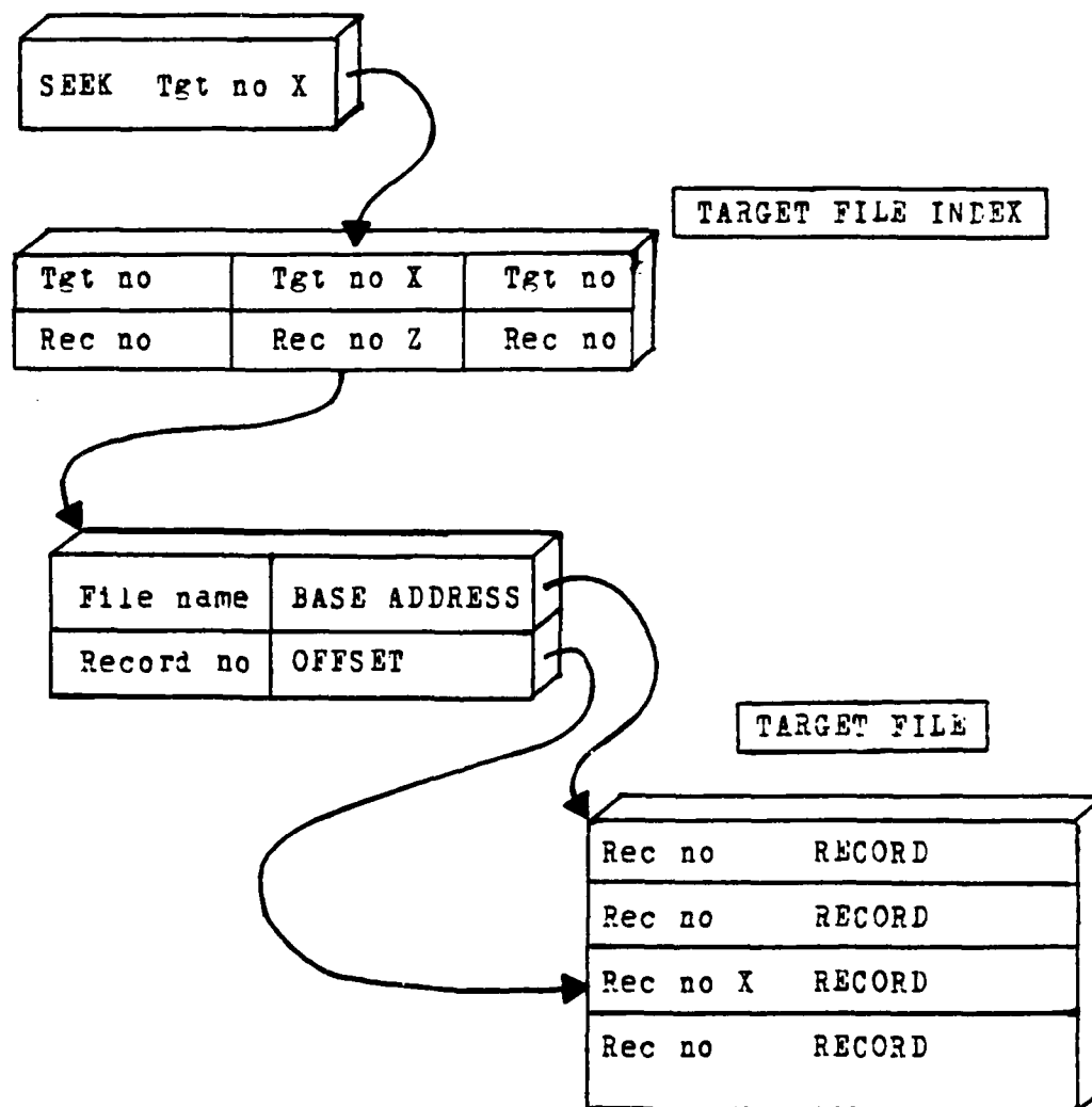
Figure 15. UCSD Pascal Random Access Capability.
