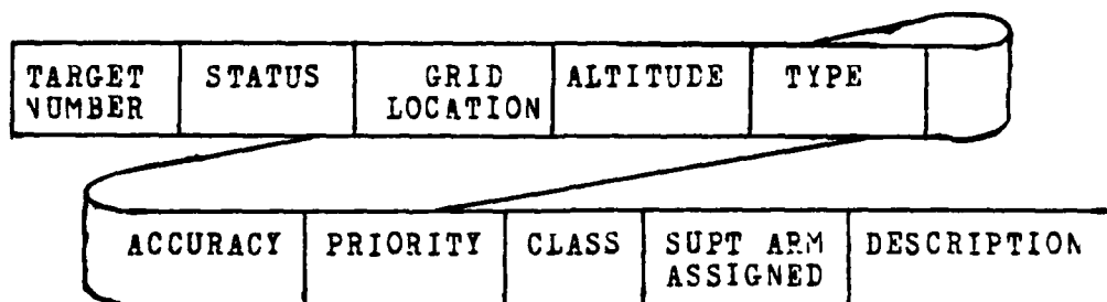
Figure 16. Data Base Query File Logical Design.
