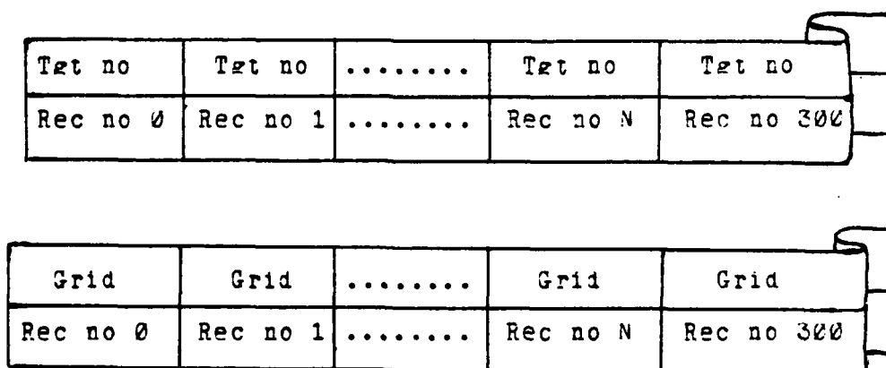
Figure 14. Target File Index Design.
