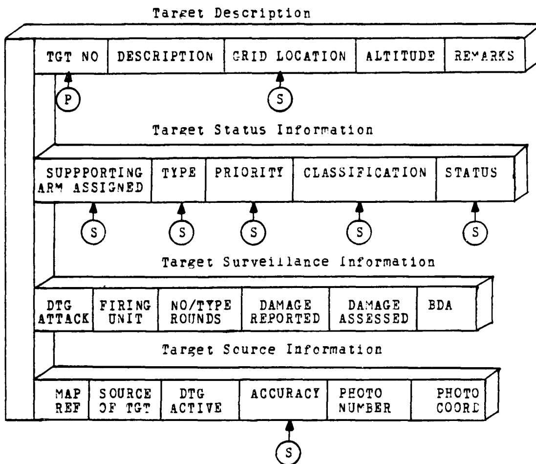
Figure 12. Logical Record Design.
