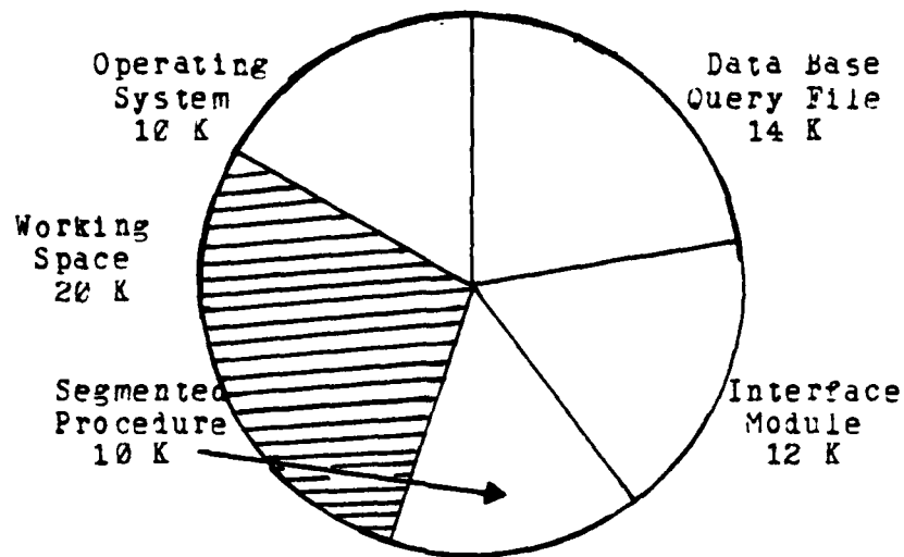
Figure 17. Main Memory Map For Data Base Queries.
