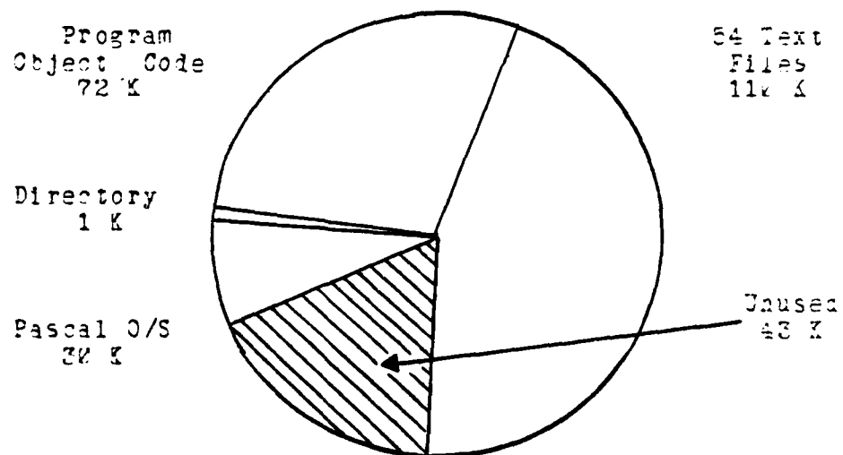
Figure 23. Actual Secondary Storage Usage.
