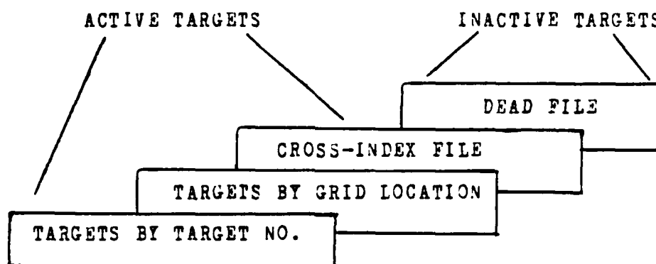
Figure 2. Target Card File Organization.
