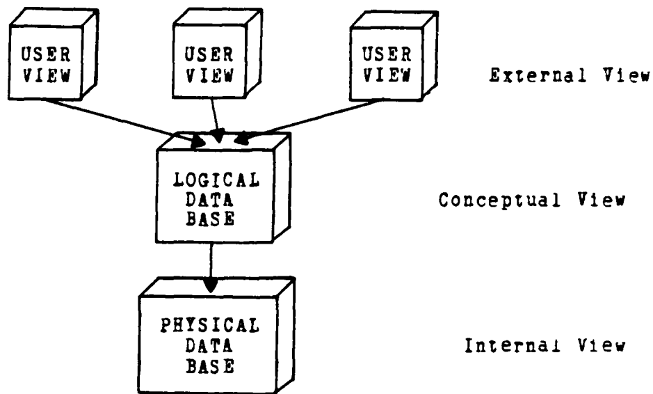
Figure 8. Data Base System Architecture.
