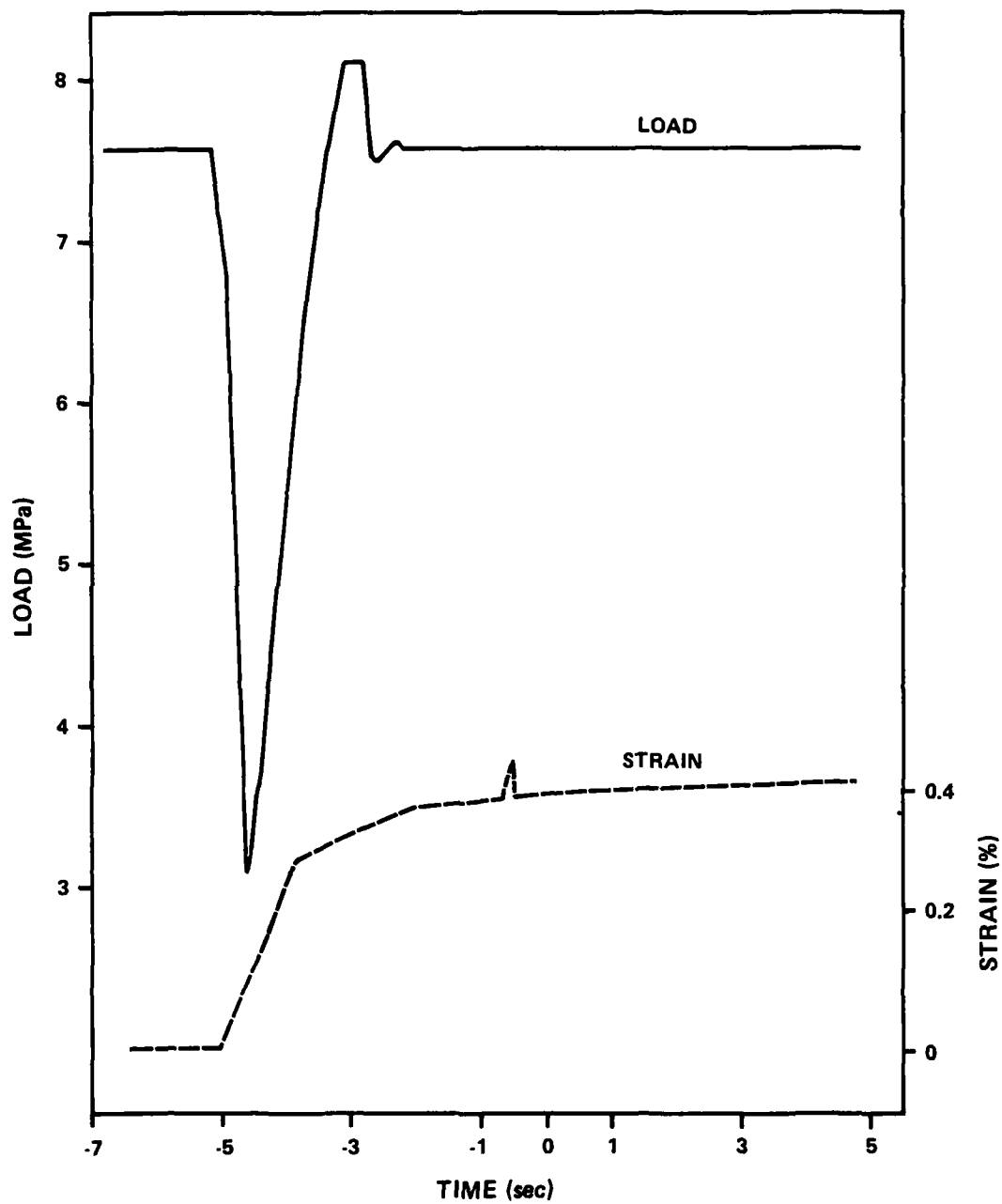
Fig. III-15 Time Required for Load Application
