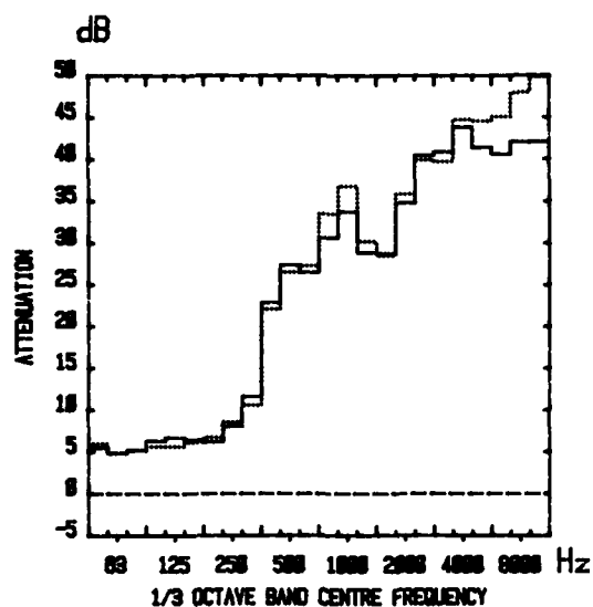
Fig 5 Left versus right ear data: Mk 4 helmet: insertion loss
