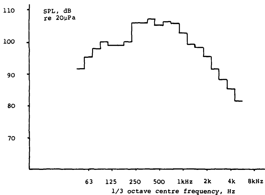
FIGURE 6: LABORATORY TEST NOISE SPECTRUM
