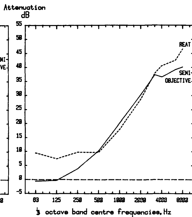
Fig 10 A comparison of REAT and semi-objective attenuation data: Mk 2/3 helmet
