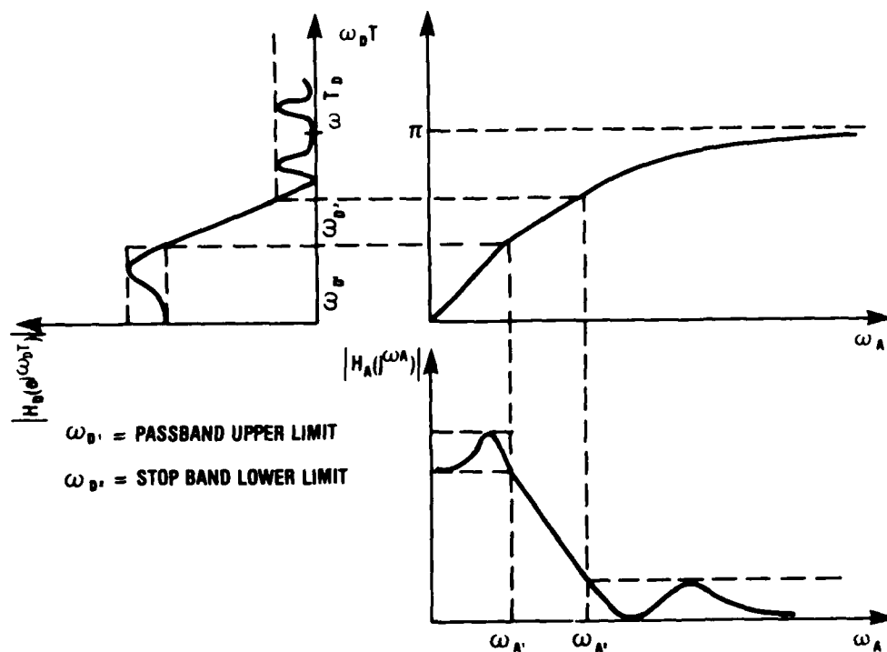
Figure 1. Bilinear transformation.
