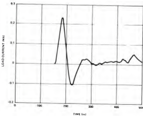
(a) LOAD CURRENT
