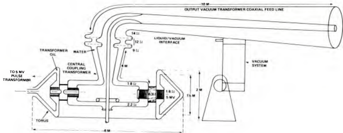
Figure 4. Proposed 1/4-MJ prototype of Camelot.
