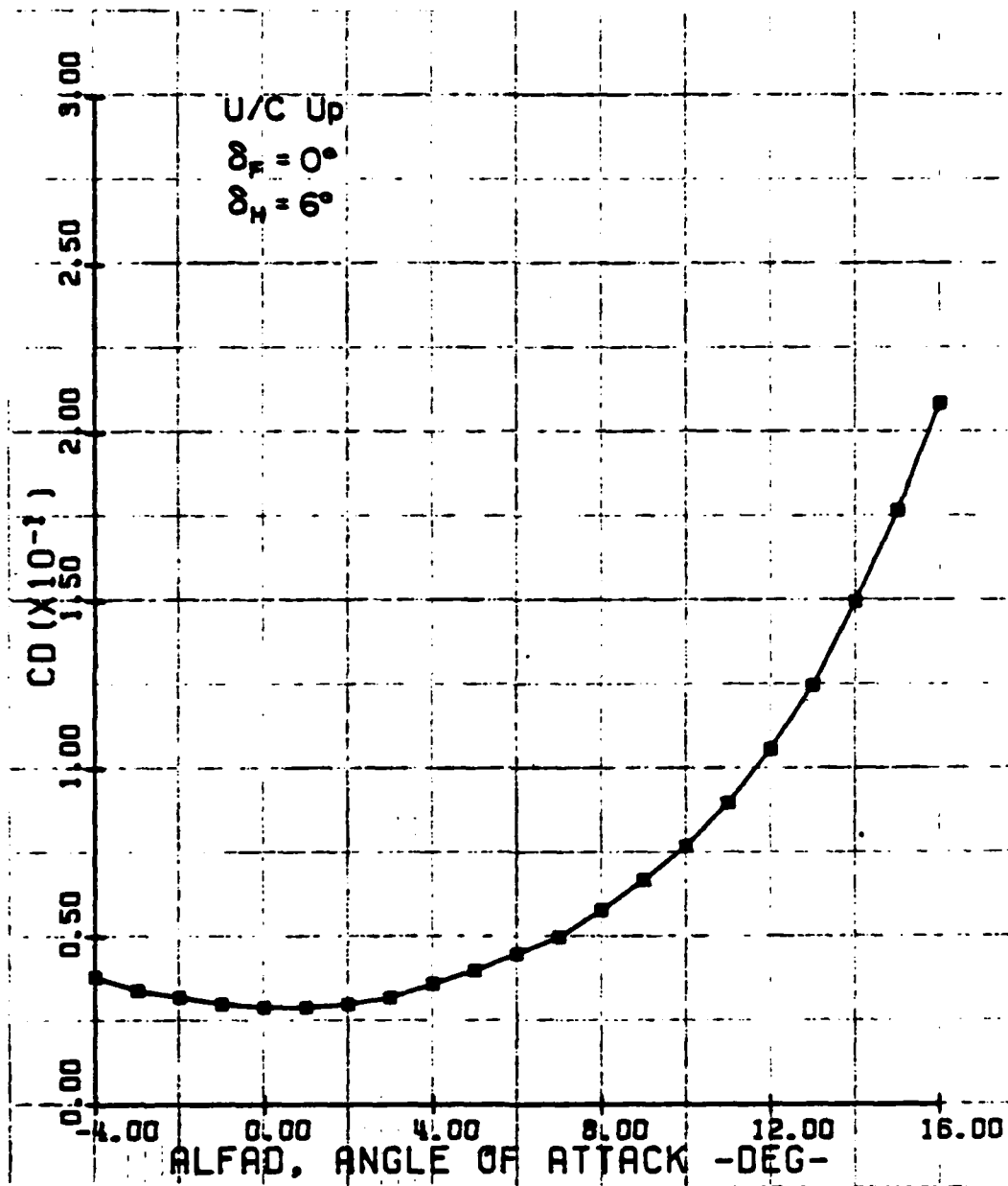
FIGURE 35 - C_{D_{wing-body}} Flaps Up, Without Wing/Jet Interaction
