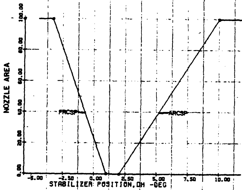
FIGURE 55 - RCS Nozzle Opening as a Function of Stabilizer Position.
