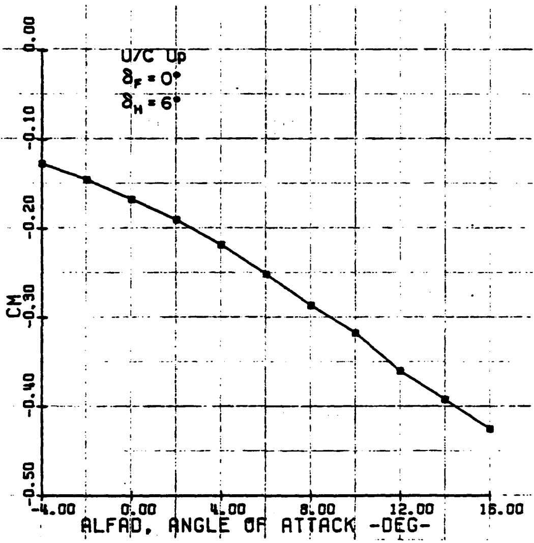
FIGURE 36 - C_{m_{wing-body}} Flaps Up, Without Wing/Jet Interaction
