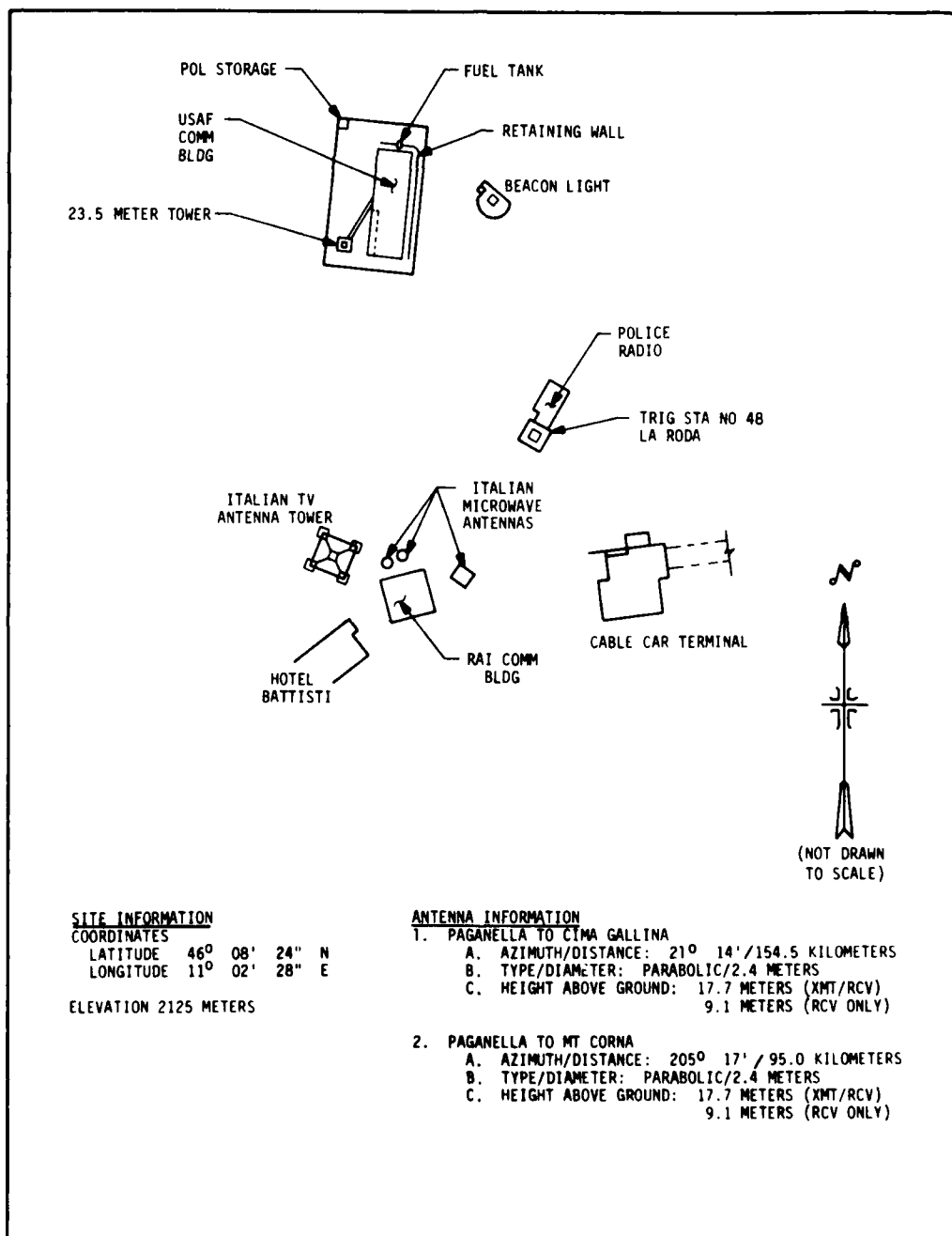
Figure 48. Paganella Site Plan
