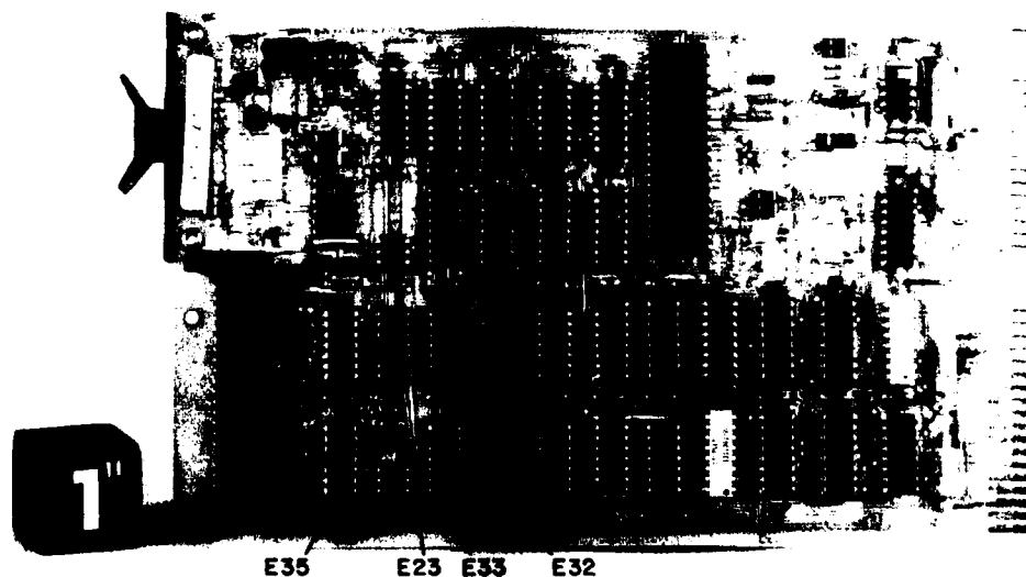
I-4. DLV-11 Modification Component Locations
