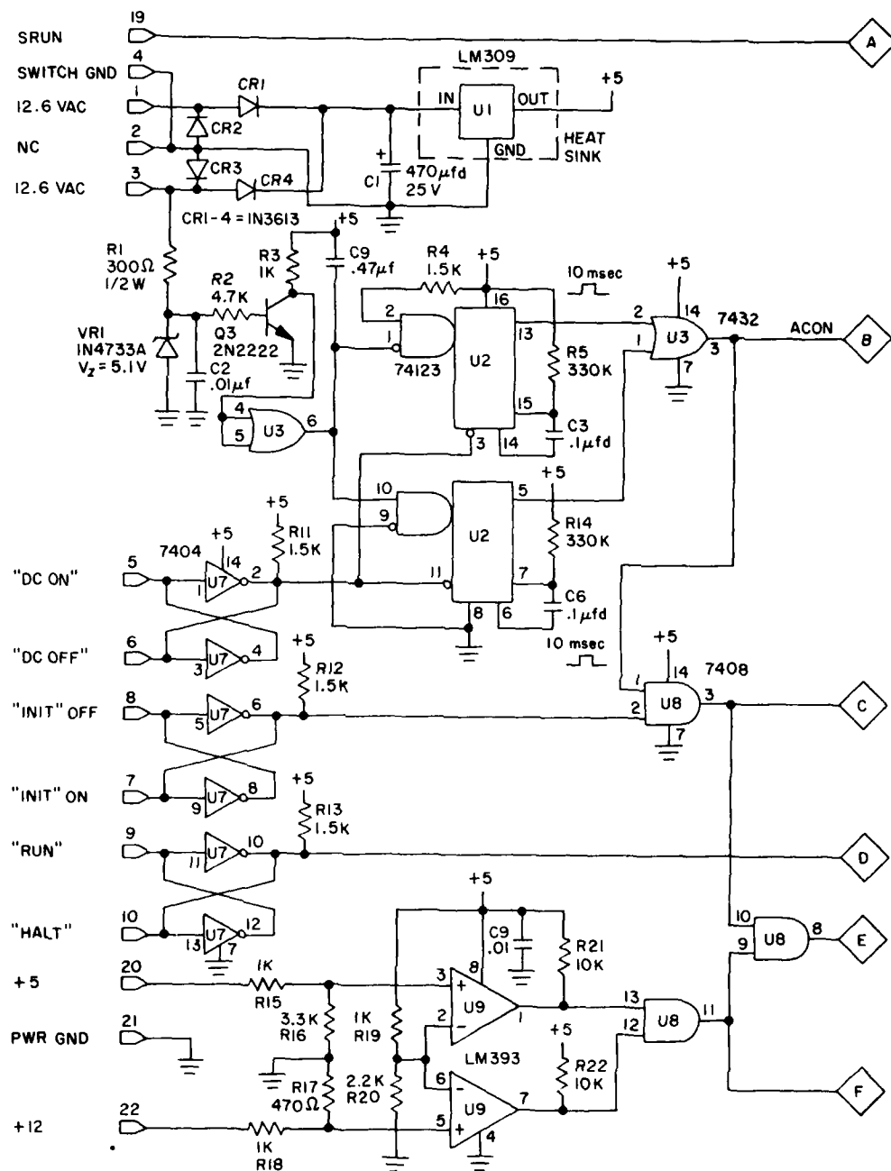
J-3. System Controller Power Control Board Schematic
