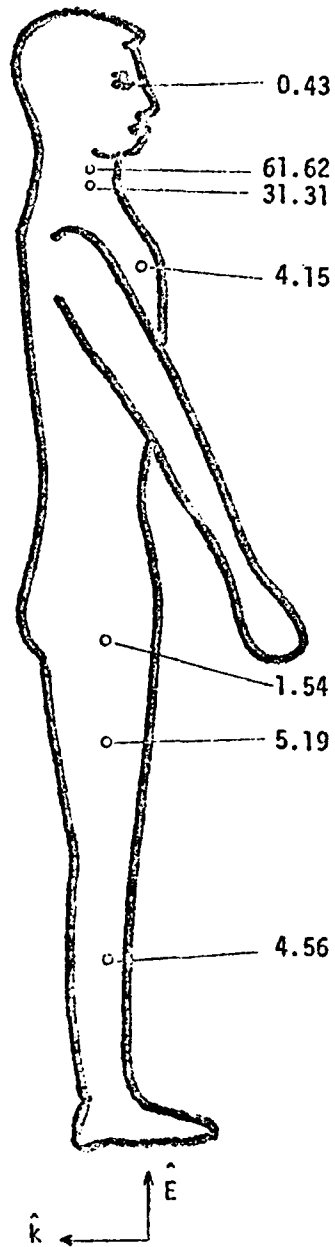
Fig. 3. Power deposition in W/kgm for 1.75 m human under \vec{E} \parallel \hat{i} resonance condition ( L/\lambda = 0.4 , 67.9 \cdot (1.75/L_m) MHz). Incident fields: 10 \text{ mW/cm}^2 .
