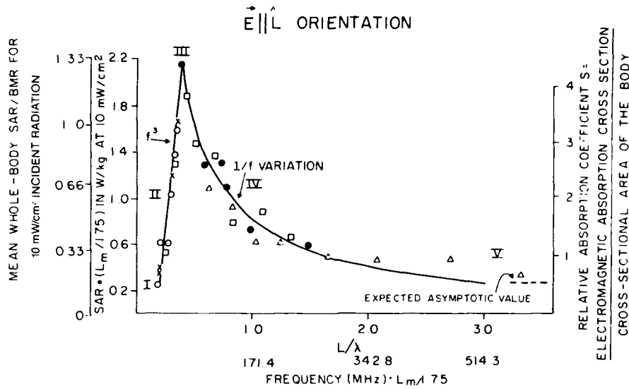
Fig. 1. Whole-body averaged SARs and the relative absorption coefficient, S_r , of saline-filled models of human beings during microwave irradiation in the free field. The E -field vector is parallel with the long axis of the model. Direction of propagation is normal to sagittal plane. Legend: \circ = prolate spheroids of (L/2b) = 6 , at 710 MHz; x = human-shaped dolls at 500 MHz (parallel-plate transmission line); \bullet = human-shaped dolls at 987 and 2450 MHz; \square = accurately proportioned figurines, 7 to 41 cm in length, at 987 MHz; \blacktriangle = the proportioned figurines at 2450 MHz.
