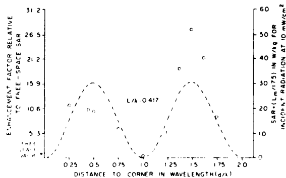
Fig. 8. Whole-body averaged SARs of a model of a human being near a 90^\circ -corner reflector. The dashed line gives values of E^2 in the absence of the model.
