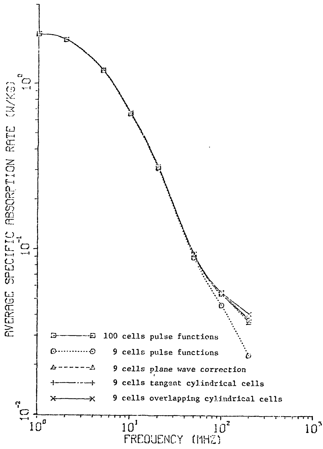
Fig. 2. Variation of average specific absorption rate with frequency for the infinite cylinder model of man.
