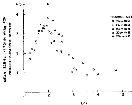
Fig. 4. Projected SARs for a human being of height L (in meters) as a function of L/\lambda . Feet are in conductive contact with ground. Sample size ( N ) is shown in parentheses in body of figure.
