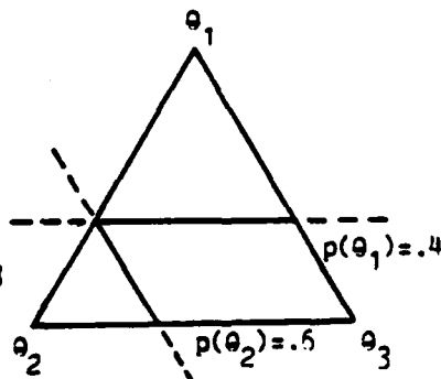
Fig. 2.3b Coherence
