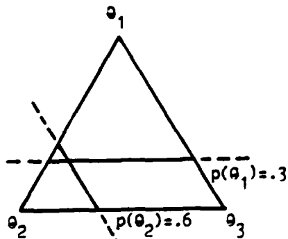
Fig. 2.3a Strict Coherence
