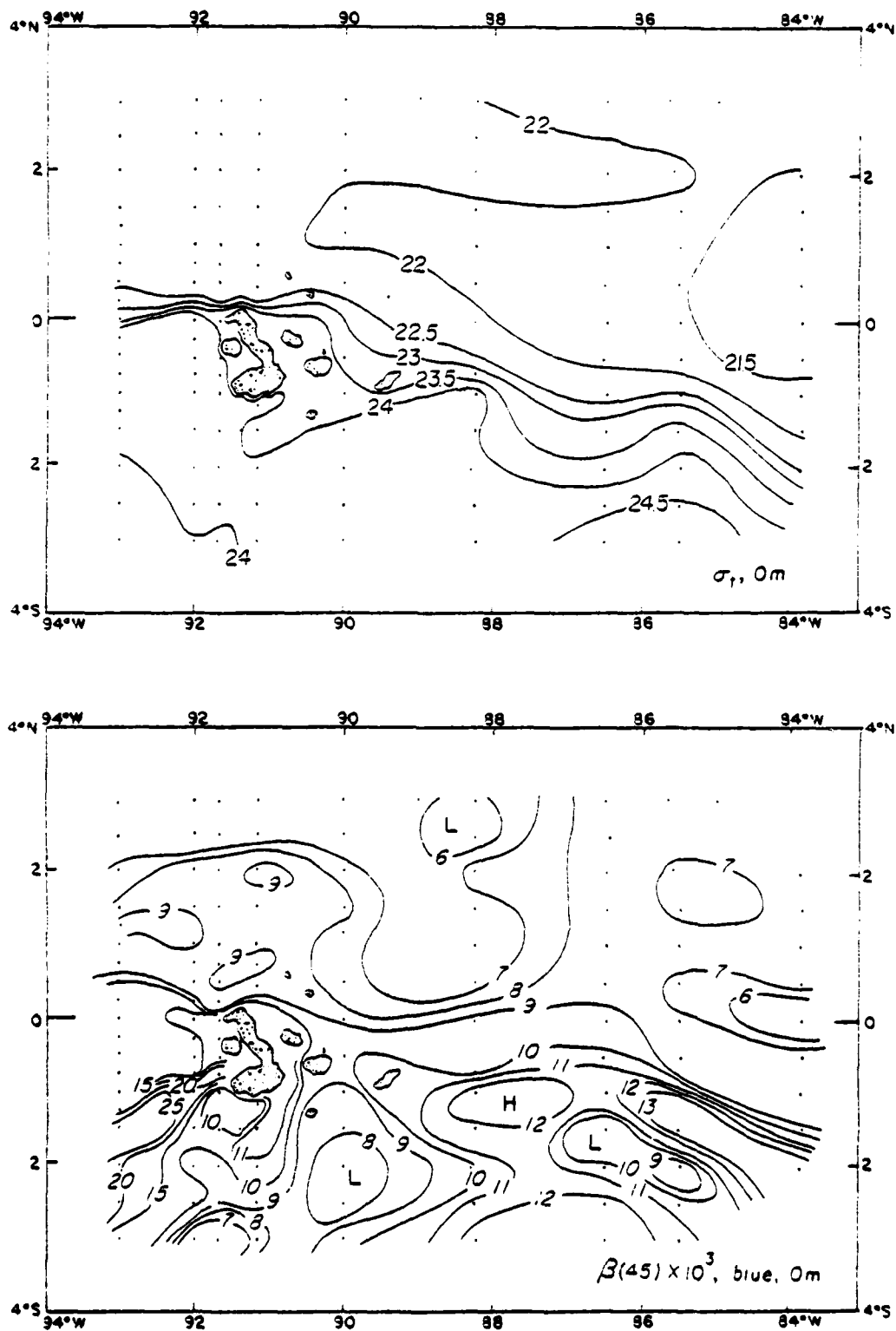
Figure 4-1. (a) Density ( \sigma_t ) in the sea surface near the Galapagos Islands. (b) Light scattering at 45° for the same region. Note scattering maximum at the front.
