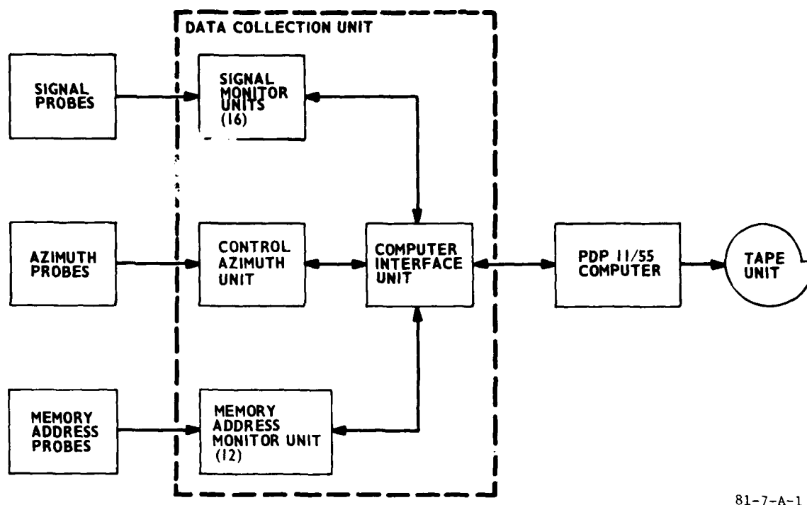
FIGURE A-1. COMPUTER PERFORMANCE MEASUREMENT SYSTEM FUNCTIONAL BLOCK DIAGRAM
