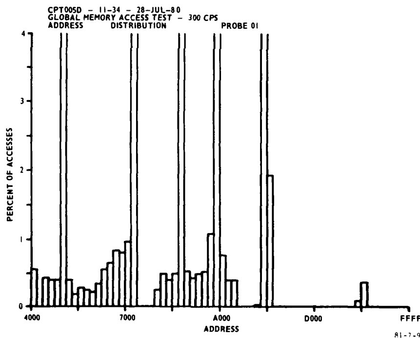
FIGURE 9. GLOBAL MEMORY ACCESS MAP, ENSEMBLE 1 PROCESSOR 2 (SS014X)
