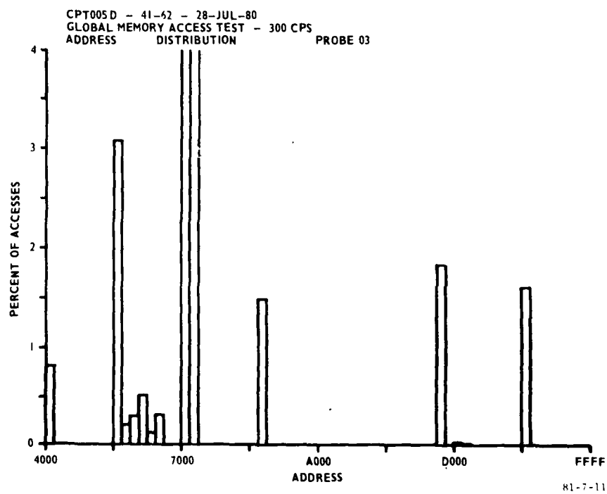
FIGURE 11. GLOBAL MEMORY ACCESS MAP, ENSEMBLE 4 PROCESSOR 4 (SS00AX)
