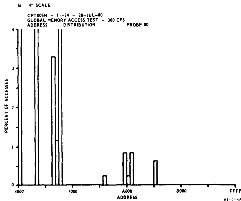
FIGURE 8. SAMPLE GLOBAL MEMORY ACCESS MAPS
