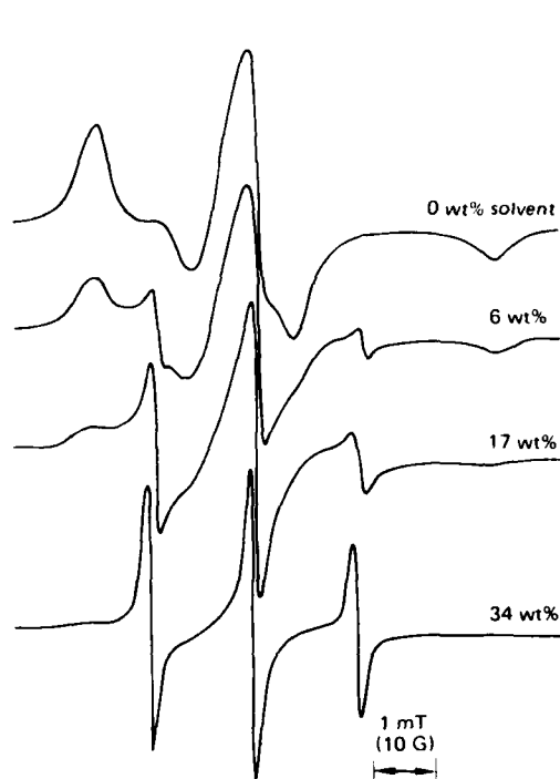
Figure 27. The effect of solvent (water) on the EPR lineshapes for the spin probe TANOL in DGEBA cured with DETA (1:3 stoichiometry).
