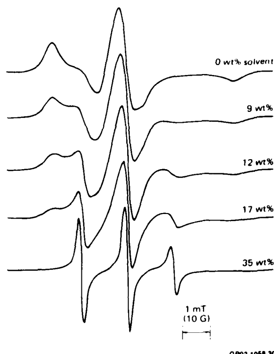
Figure 28. The effect of solvent (water) on the EPR lineshapes for the spin probe TANOL in samples of MY720 cured with DETA (1:5 stoichiometry).
