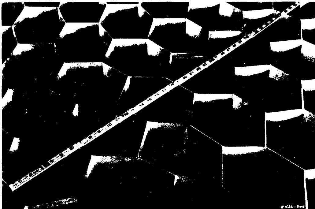
Photo 5. Close-up view of installed grids, test section 3
