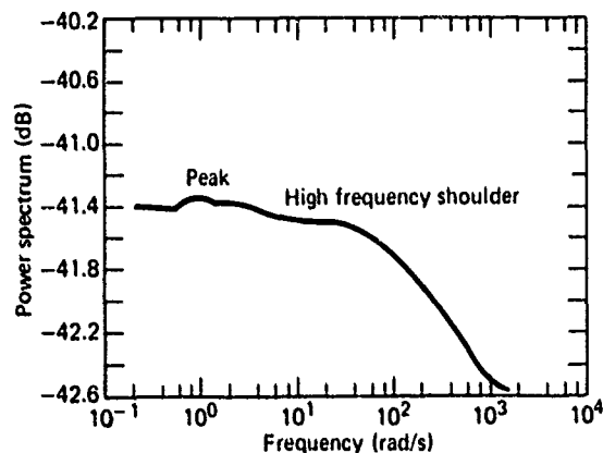
Fig. 4 Glitter power spectrum, u_* = 48 cm/s.
