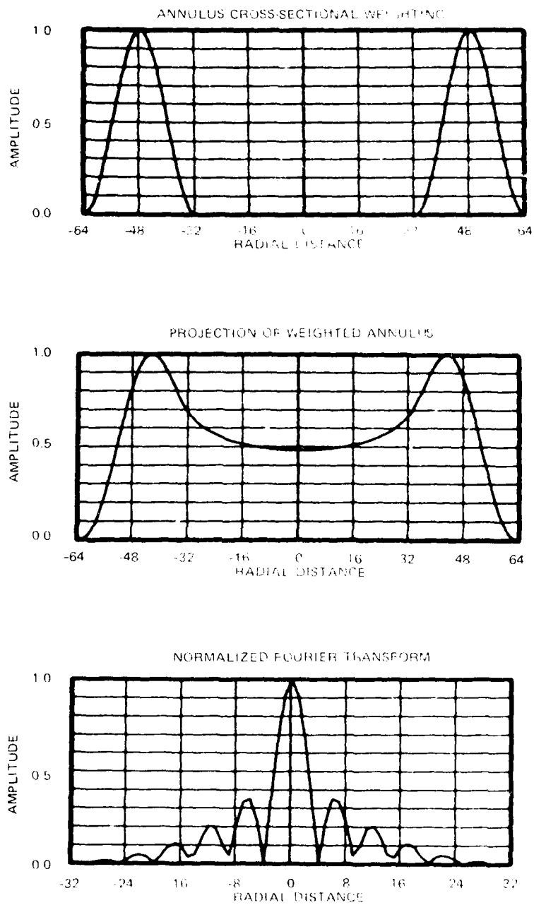
Figure A-4 Annulus Spectrum With \cos^2(x) Tapered Weighting
