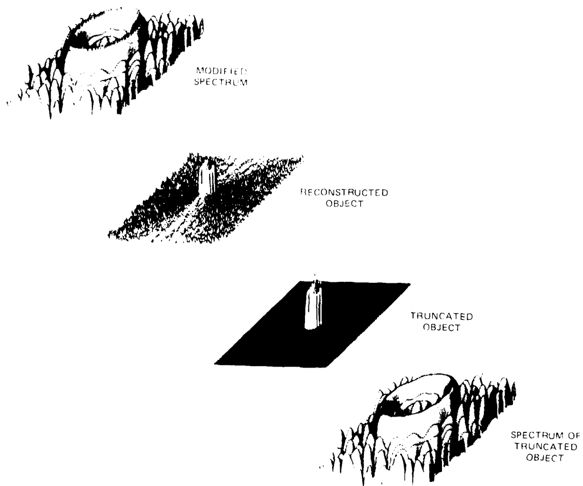
Figure 5-11. Spatial and Spectral Responses for Tenth Iteration of the Algorithm Applied to a Ring Spectrum (Radius of Object Truncation = 1.5)
