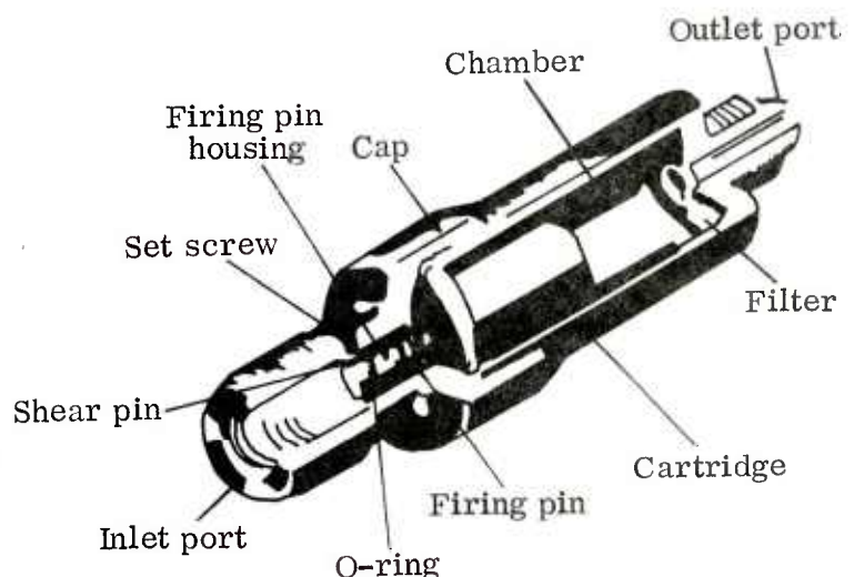
Figure 44. Gas Operated Initiation MK 10 Mod 0
