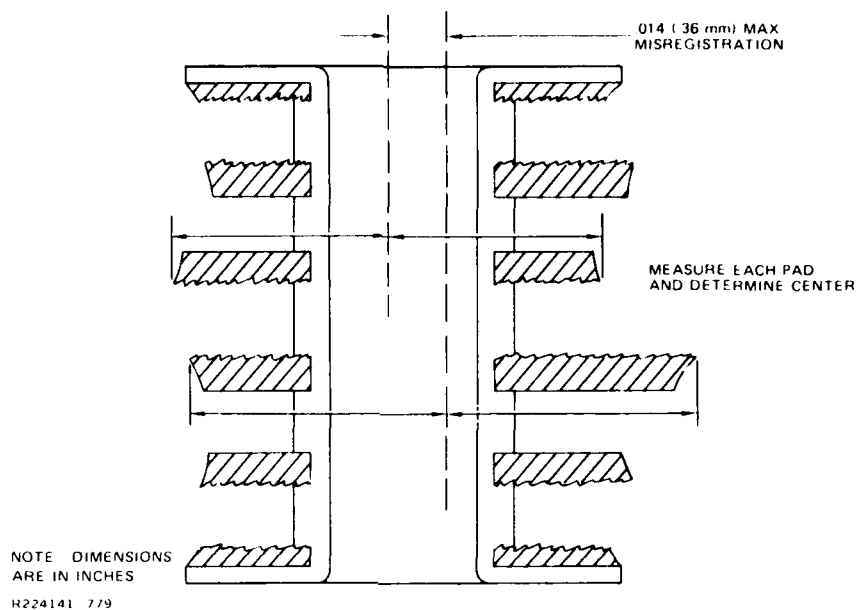
Layer to layer registration.
