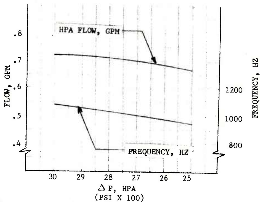
Figure 3-11. HPA Flow & Frequency Versus HPA \Delta P , Constant Resistive Load
