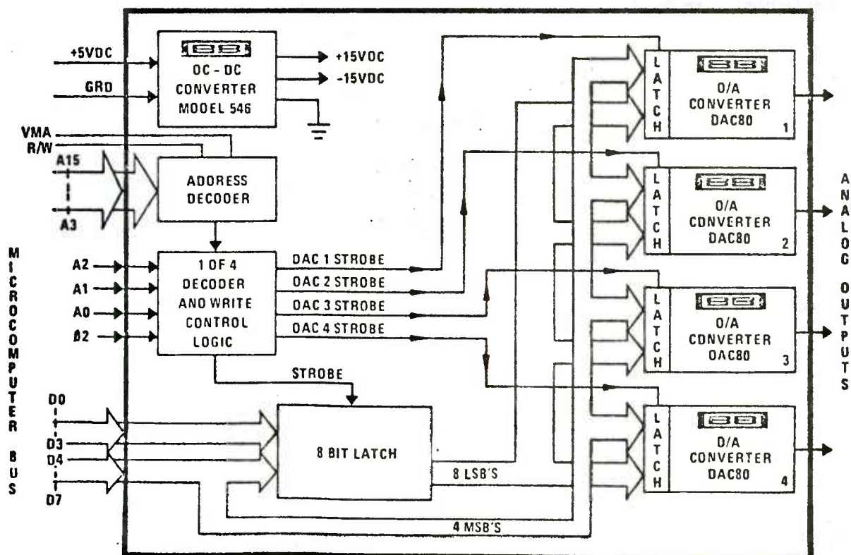
Figure A-5. Digital to Analog Converter - MP7104
