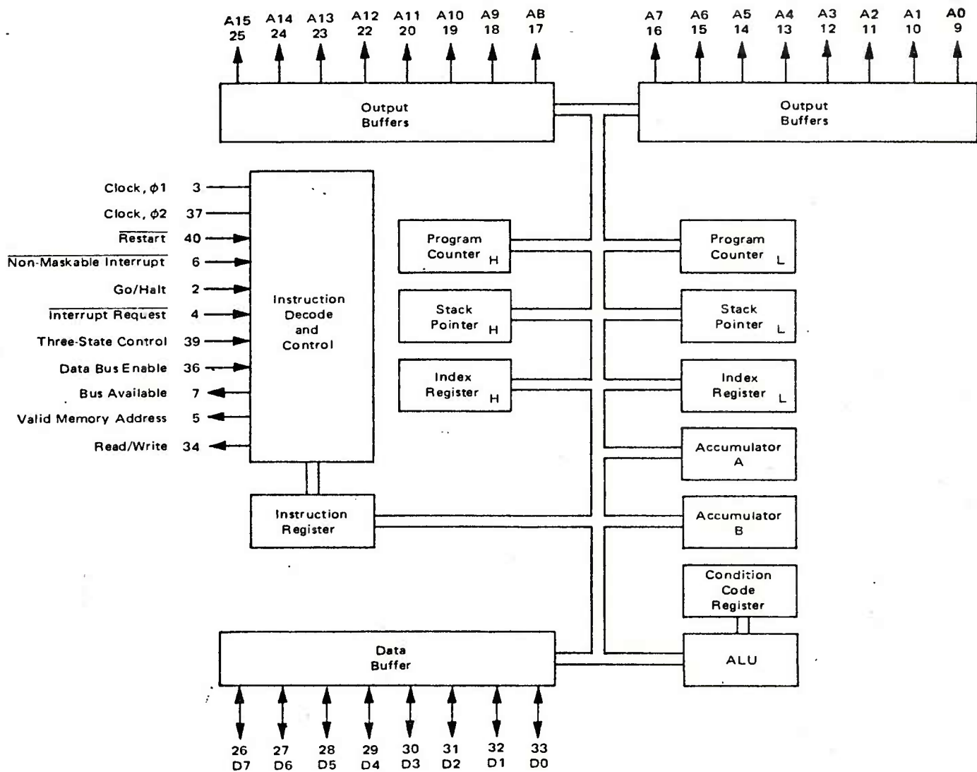
Figure A-3. Microprocessor Unit Organization (MC 6800)
