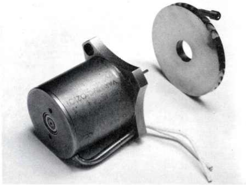
Figure 2-4. HPA Turbine Wheel and Alternator
