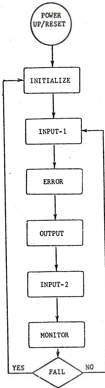
Figure 2-10. DFBL Microcomputer Program Flow Chart
