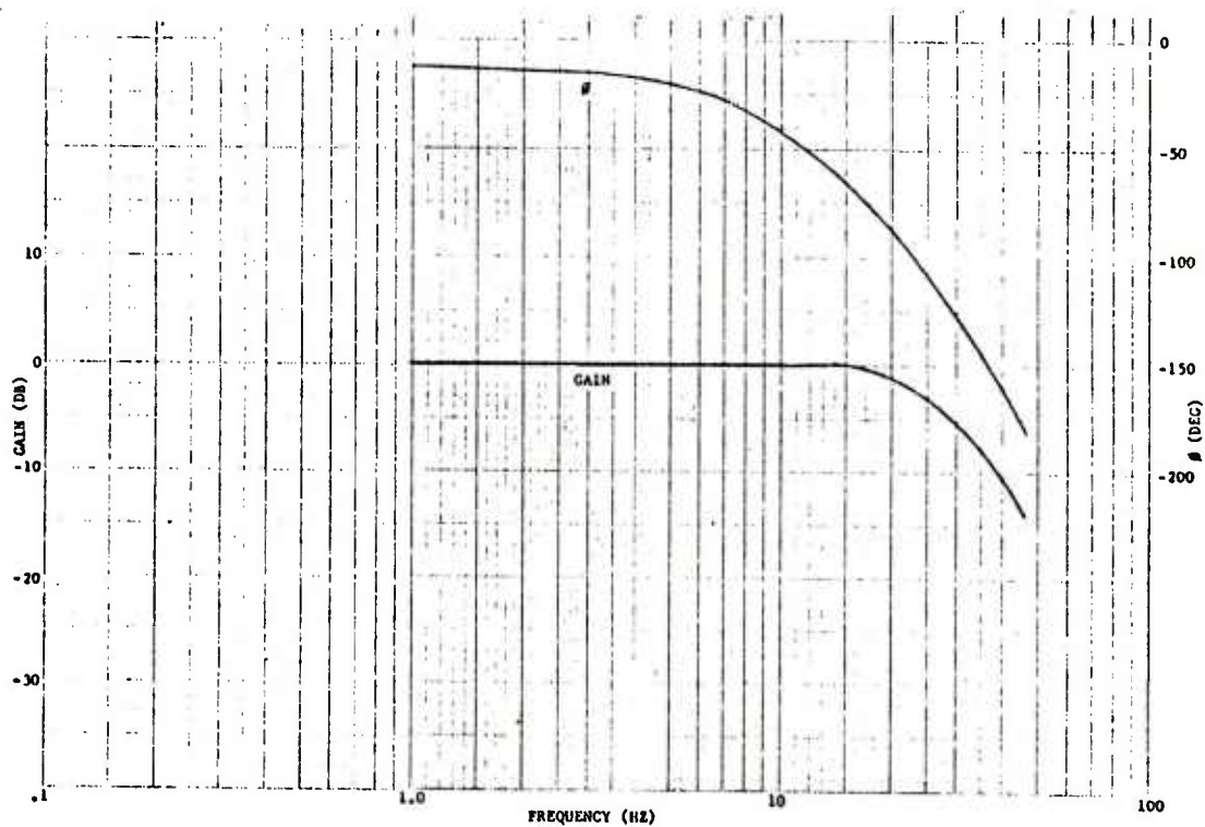
Figure 4-3. Frequency Response, AFCAS Designed For Direct Digital Drive
