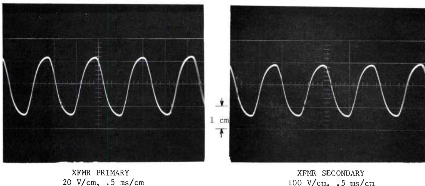
Figure 3-12. Transformer Primary and Secondary Voltage Waveforms, 2500 PSI FPA \Delta P
