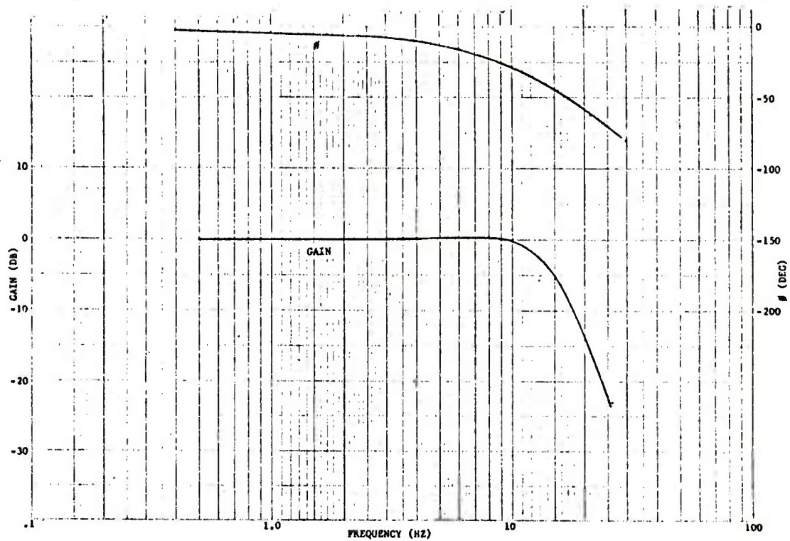
Figure 4-2. AFCAS Frequency Response
