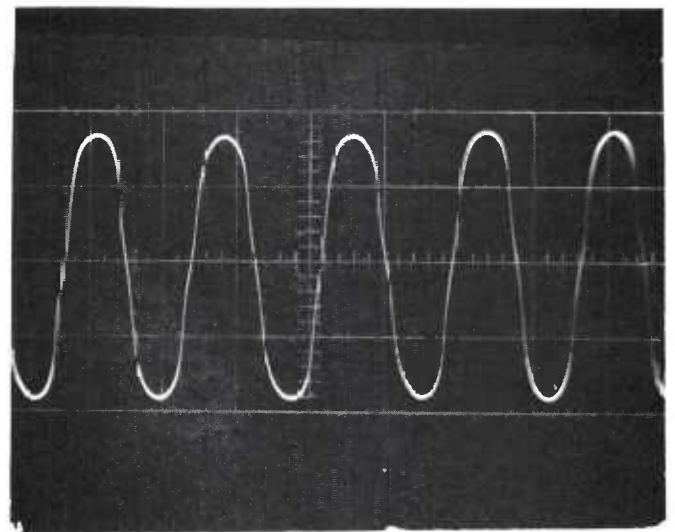
XFMR SECONDARY, I = 0a 100 V/cm, .5 ms/cm
