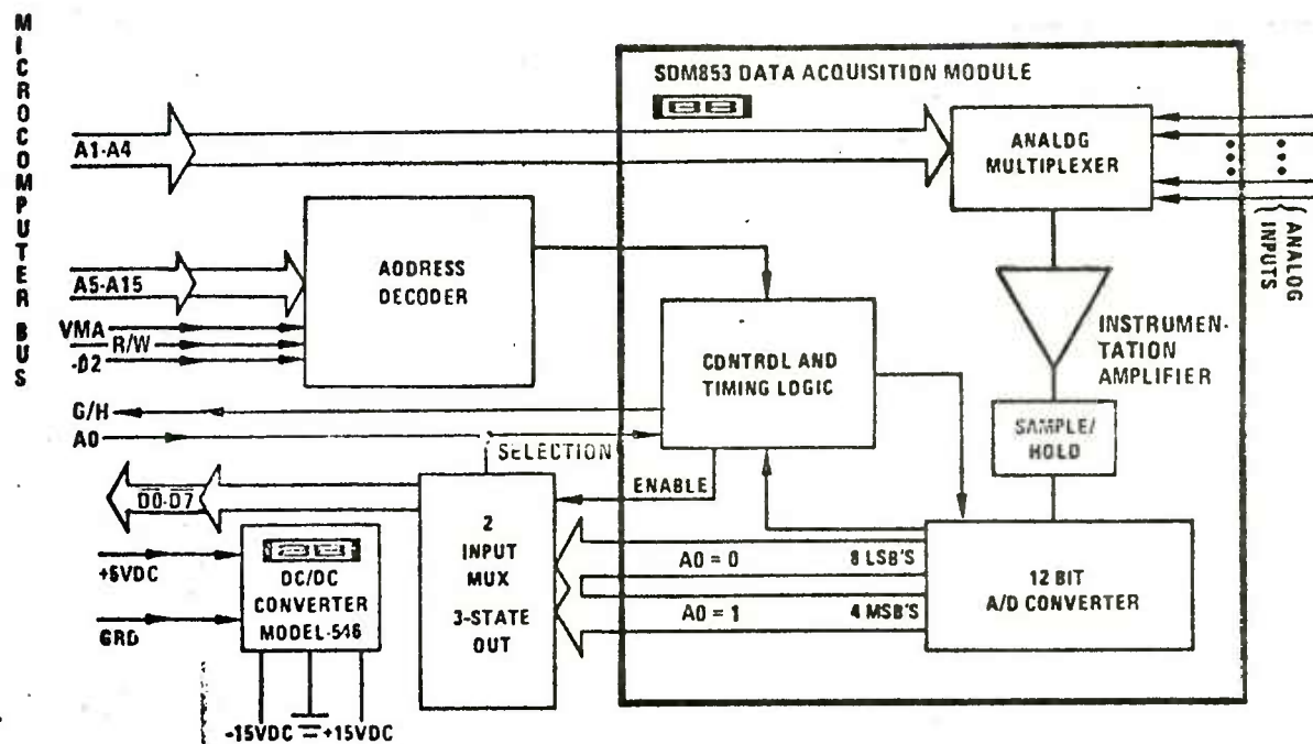
Figure A-4. Analog to Digital Converter - MP7208/7216
