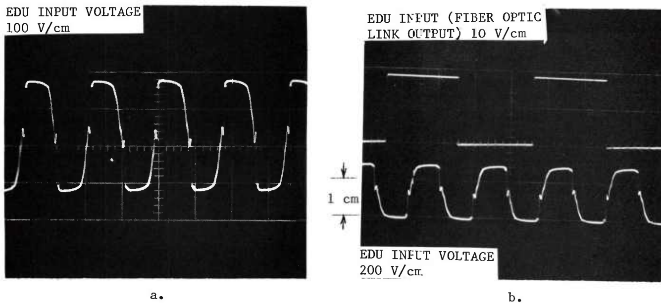
Figure 3-17. EDU Input Voltage Waveform, System Null (Microcomputer PWM Output @ 50% Modulation)
