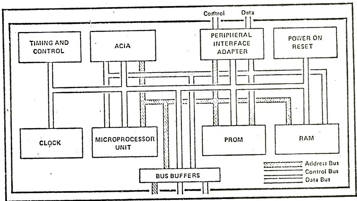
Figure A-1.. Monoboard Microcomputer Block Diagram
