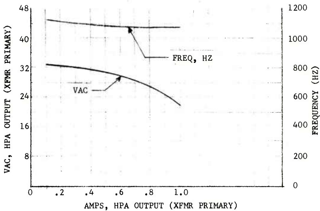
Figure 3-6. HPA VAC & Frequency Versus HPA Output Current
