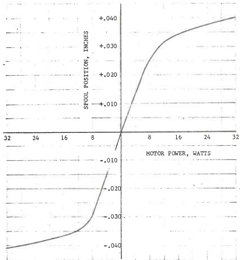
Figure 4-1. Torque Motor Characteristics
