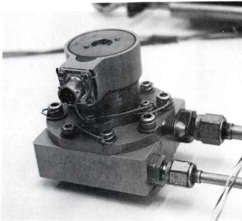
Figure 2-5. HPA Assembly
