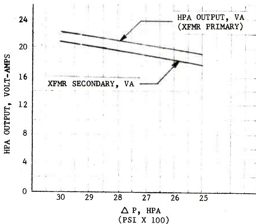
Figure 3-10. HPA VA Output Versus HPA \Delta P , Constant Resistive Load
