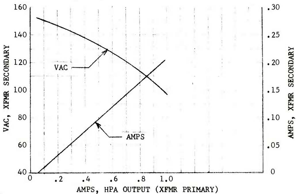
Figure 3-7. Transformer Secondary VAC & Current Versus HPA Output Current (Transformer Primary)
