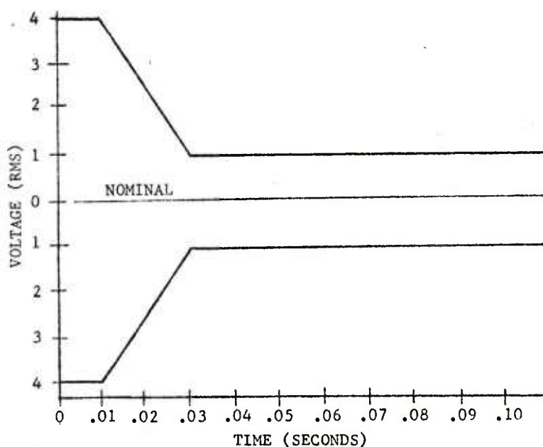
Transient and Steady State Regulation @ Rated Capacity
