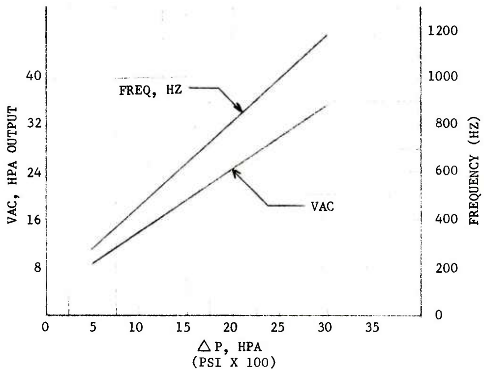
Figure 3-2. HPA VAC & Frequency Versus HPA \Delta P , No Load
