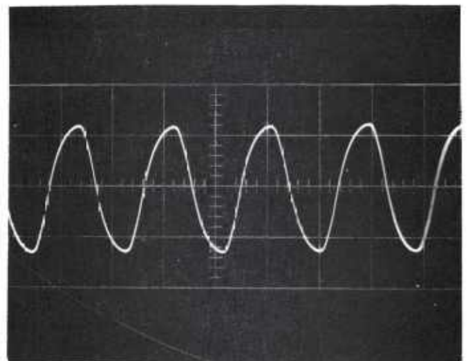
XFMR SECONDARY, I = .21a 100 V/cm, .5 ms/cm
