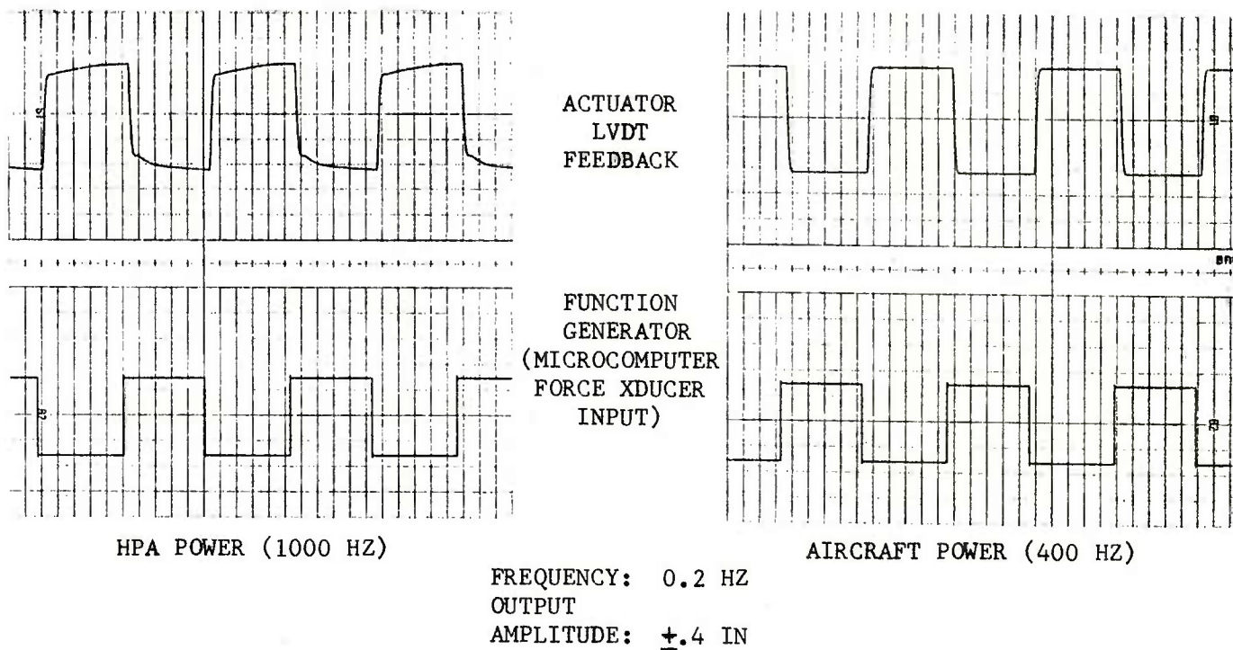
Figure 3-23. Step Input Response, Flight Gain Configuration, DFBL Mode
