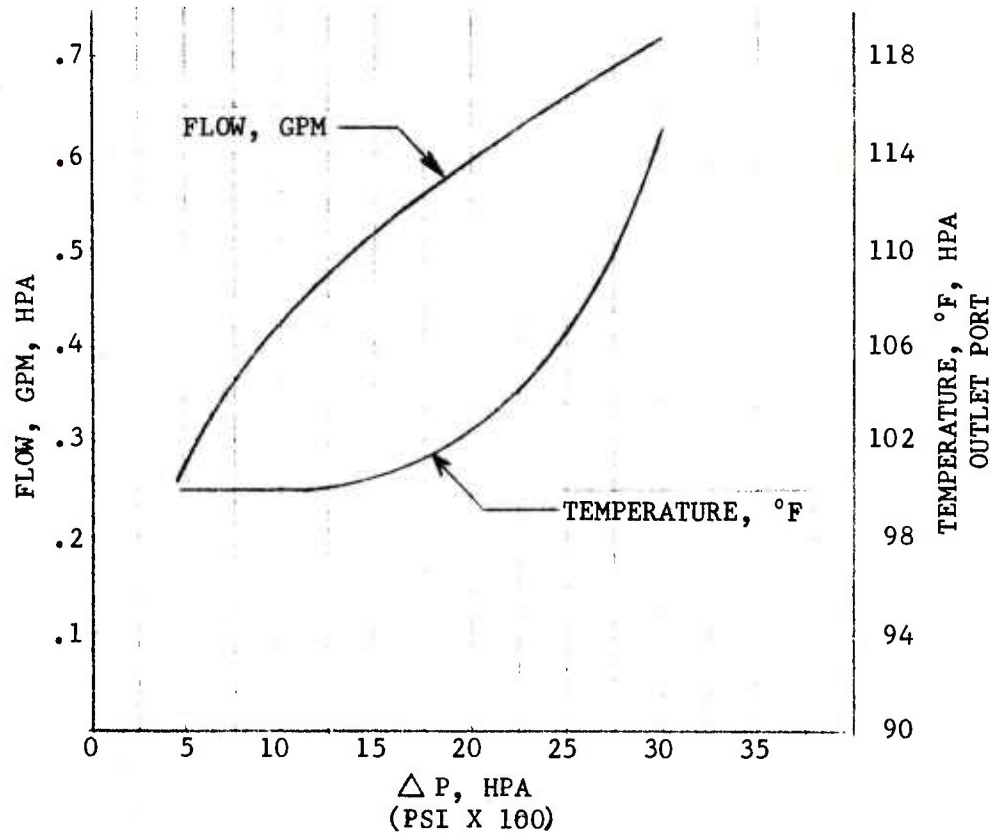
Figure 3-3. HPA Fluid Flow & Temperature Versus HPA \Delta P , No Load
