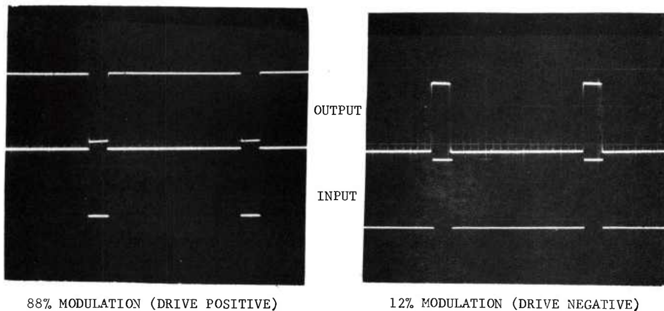
Figure 3-16. Fiber Optic Link Input/Output Waveforms, Static Gain Test
