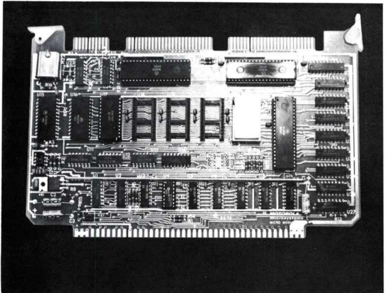
Figure A-2. Monoboard Microcomputer
