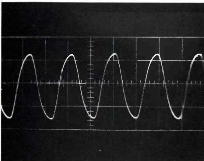
XFMR PRIMARY, I = 1.0a 20 V/cm, .5 ms/cm
