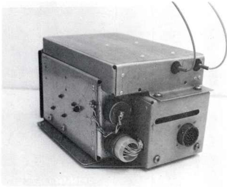
Figure 2-6. EDU With Fiber Optic Cables Attached
