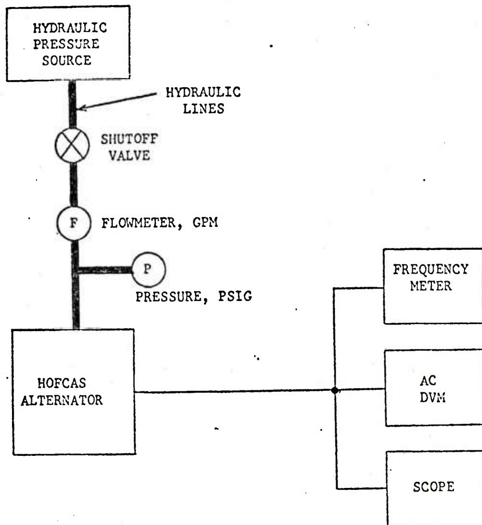
Figure 3-1. HPA No-Load Test Setup
