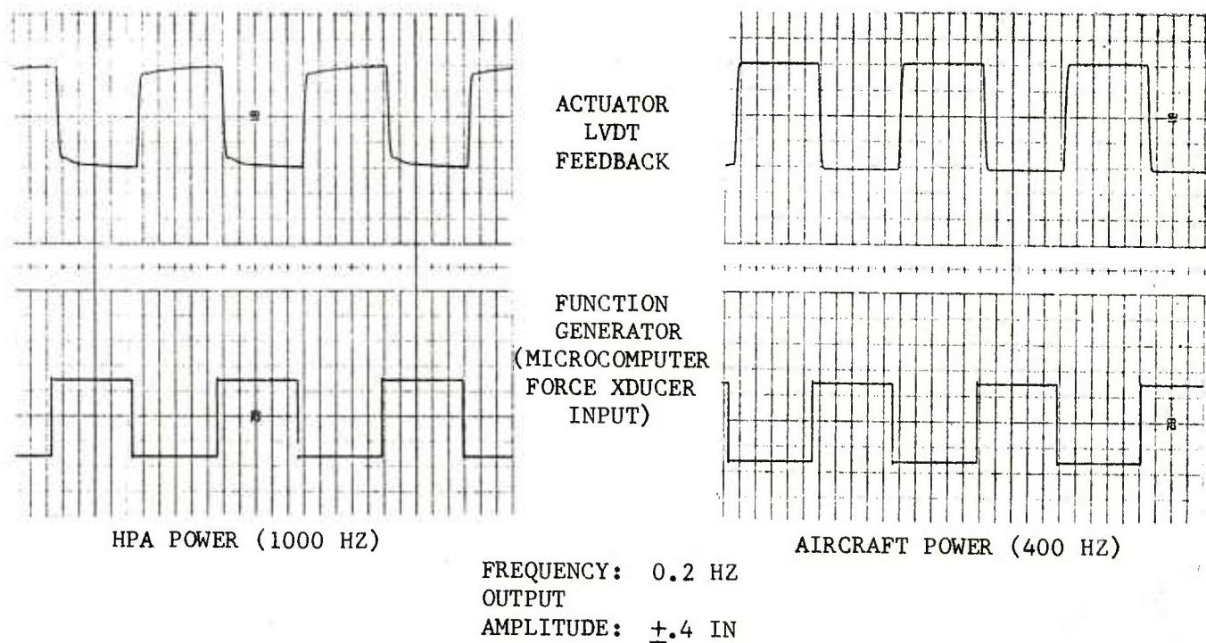
Figure 3-24. Step Input Response, Flight Gain Configuration, DFBW Mode
