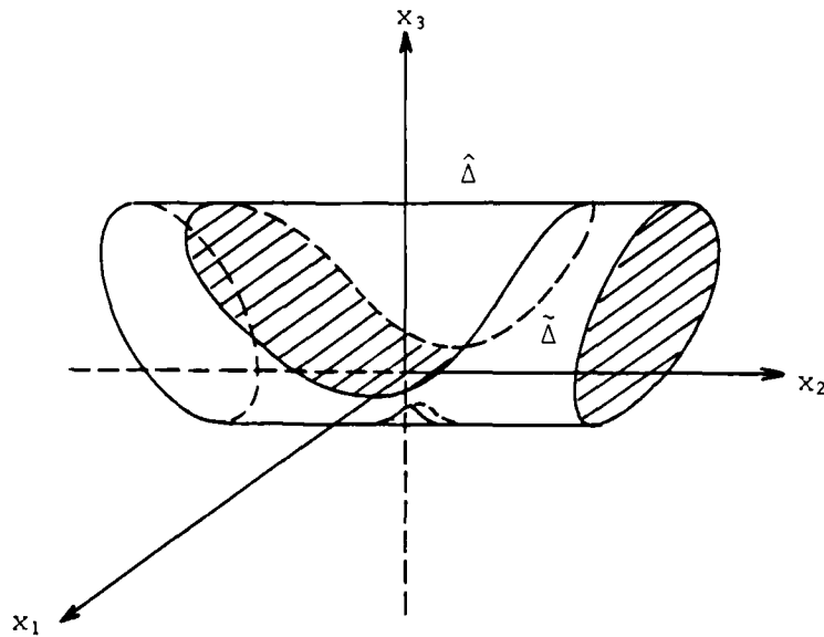
Figure 3.5 Attractors \hat{\Delta} and \tilde{\Delta} of (3)
