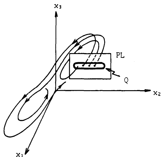
Figure 4.4 First Return Mapping
