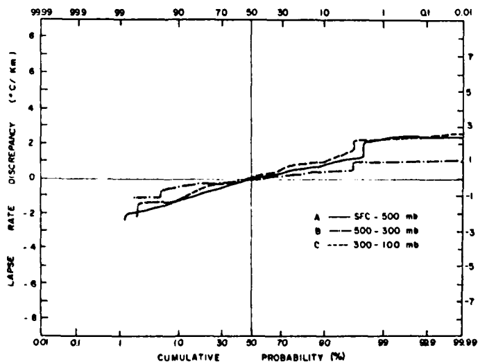
Fig. 33. Cumulative frequency distributions of discrepancies in the lapse rate of temperature within the layers surface to 500 mb, 500 to 300 mb, and 300 to 100 mb for Area II (Caribbean).
