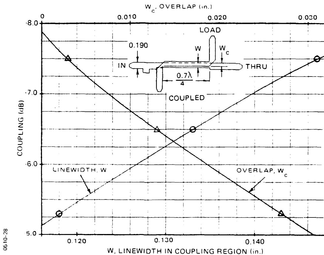
Figure 5-7. Design curve for modified \lambda/4 overlap directional coupler
