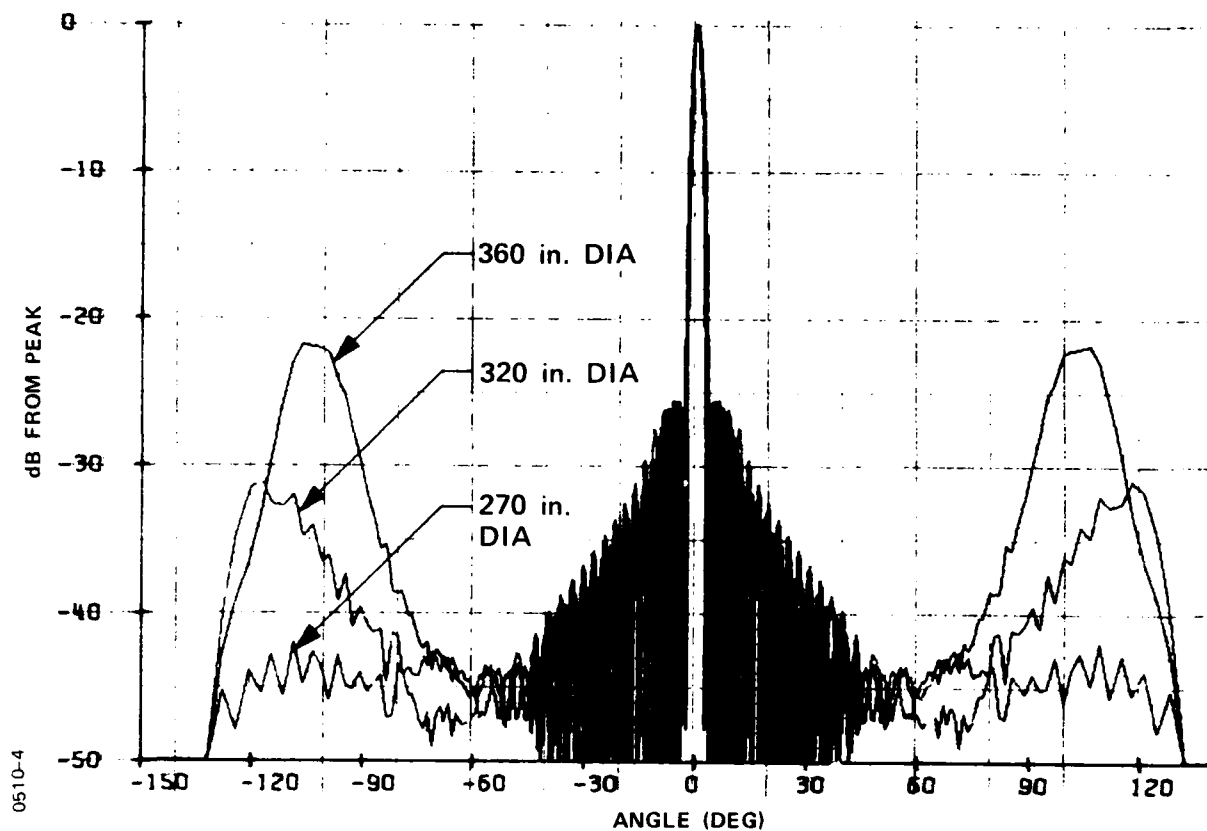
Figure 3-4. Computed azimuth patterns: 200 elements, 90° sector, -25 dB Taylor illumination
