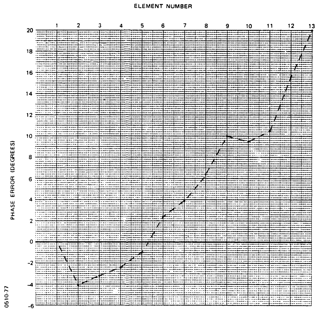
Figure 6-30. Phase error versus element number at 1.03 GHz
