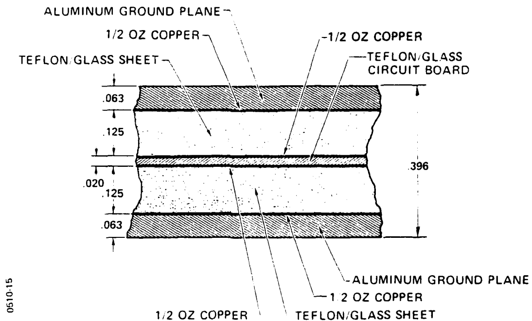
Figure 3-15. Three-layer stripline configuration
