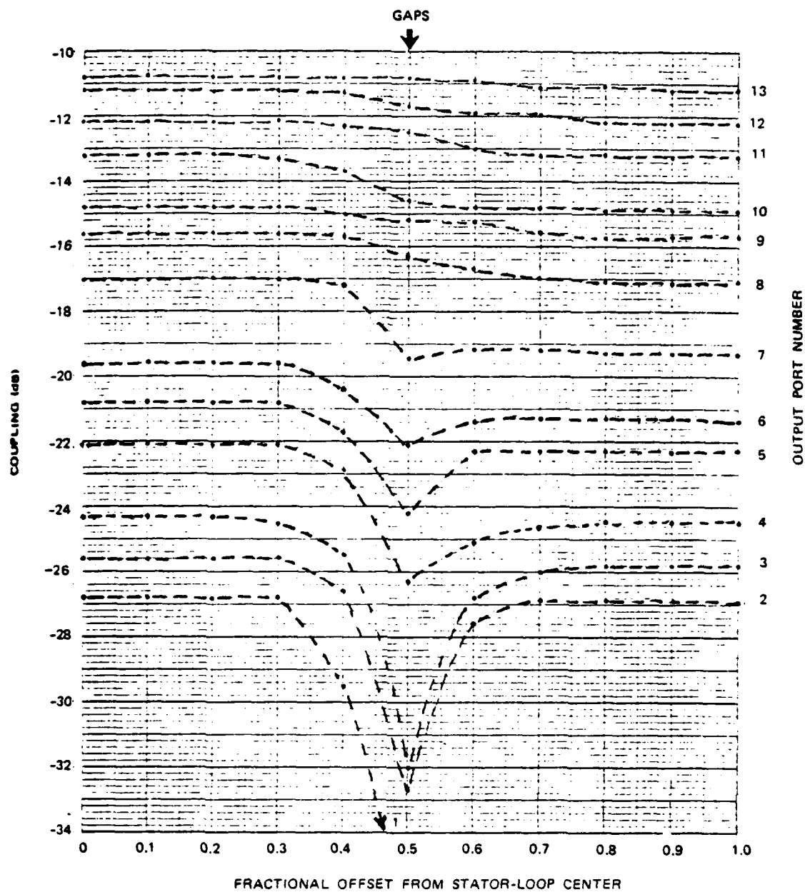
Figure 6-27. Measured loop-coupled amplitude versus offset
