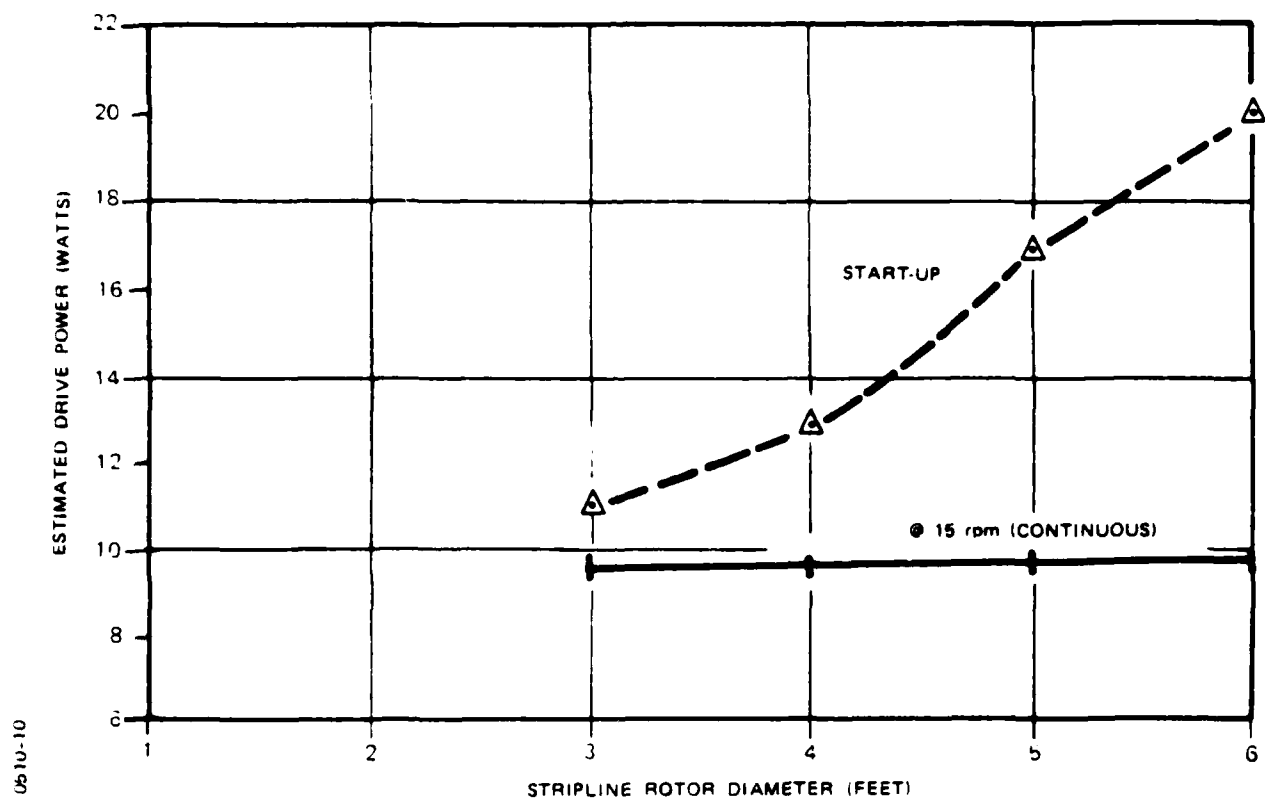
Figure 3-10. Drive power required as a function of stripline rotor diameter
