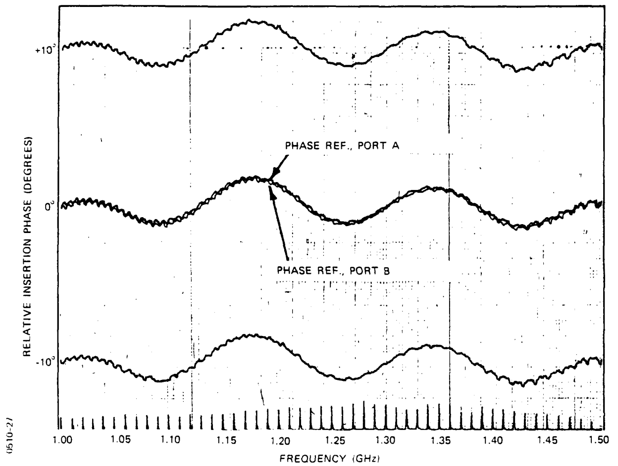
Figure 5-6. Phase difference between output ports A and B
