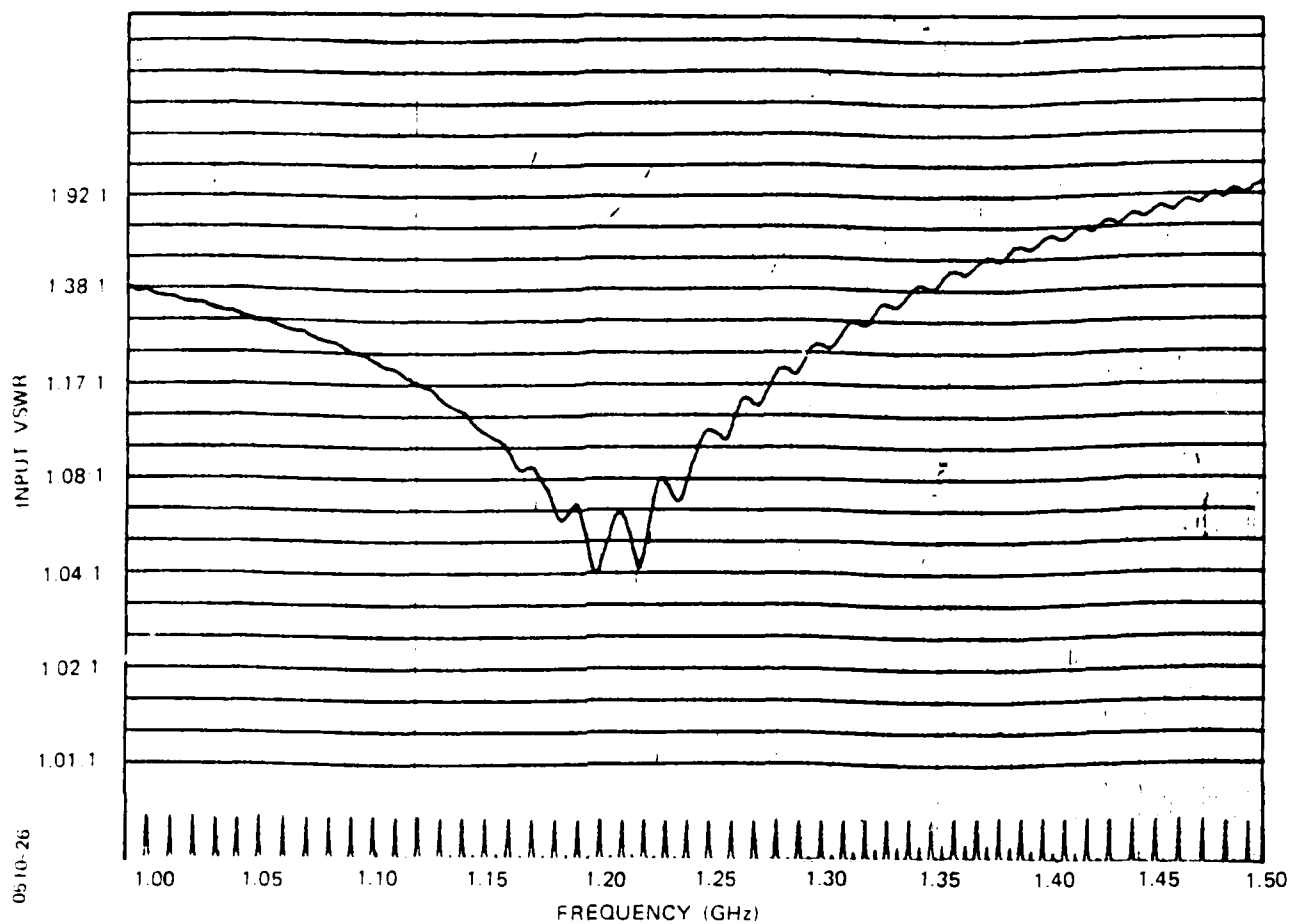
Figure 5-5. VSWR vs frequency of annular rotary coupler
