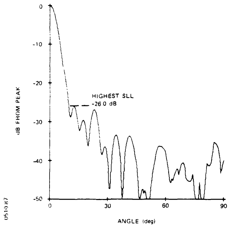
Figure 6-40. Computed azimuth pattern at 1.03 GHz
