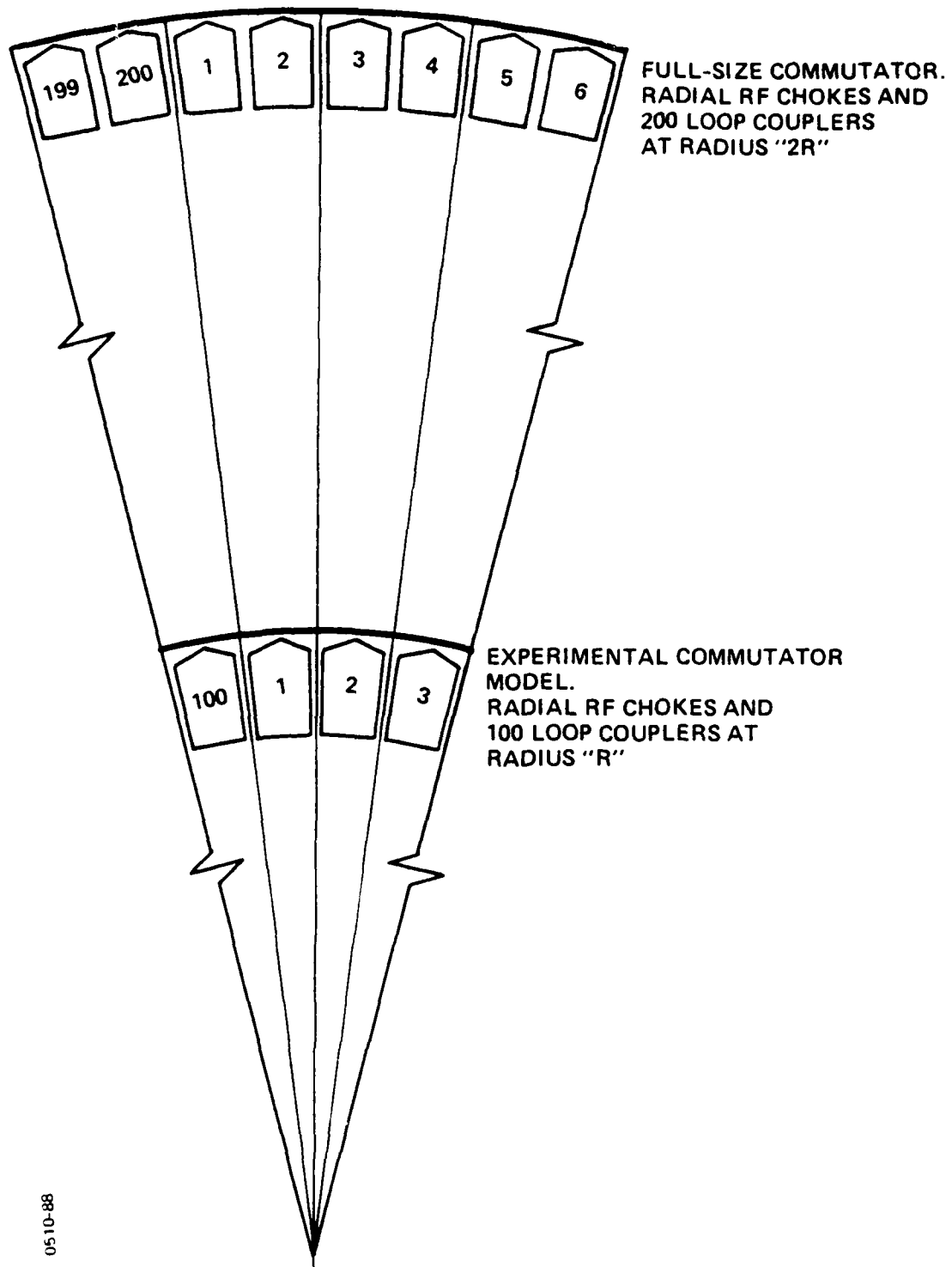
Figure 7-1. Two-fold radius increase for 200 loop couplers
