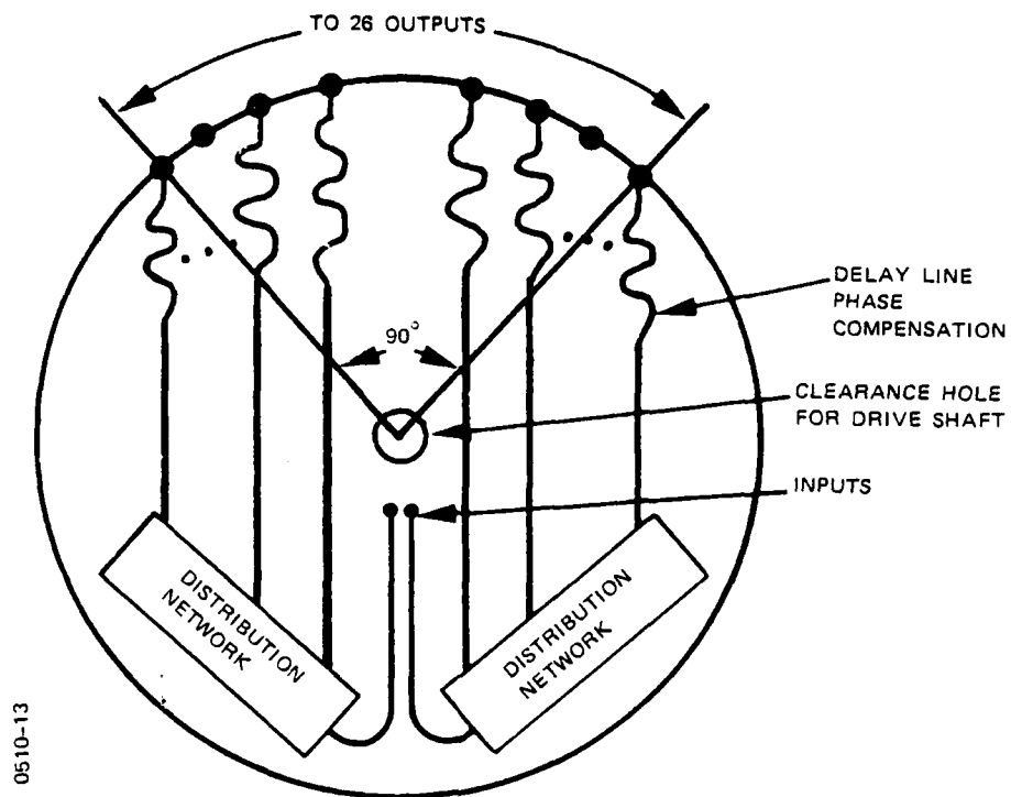
Figure 3-13. Schematic of stripline feed network
