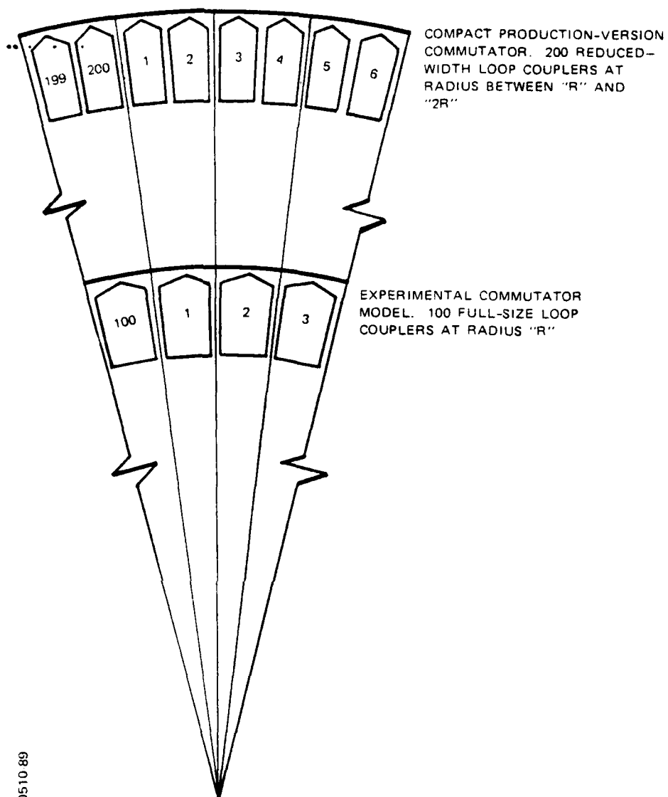
Figure 7-2. Reduced-width loop couplers to minimize radius of commutator
