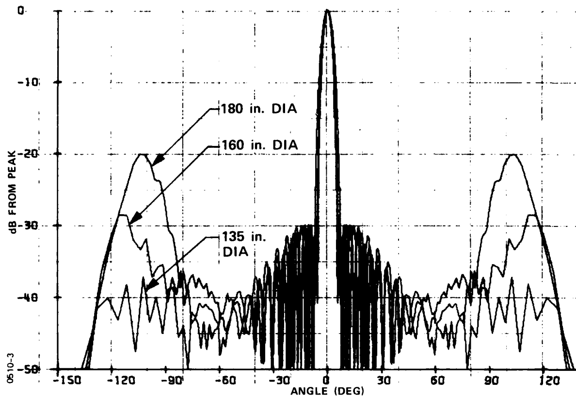
Figure 3-3. Computed azimuth patterns: 100 elements, 90° sector, -29 dB Taylor illumination
