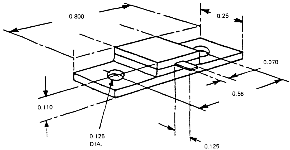
Figure 5-11. Flanged 50-ohm load
