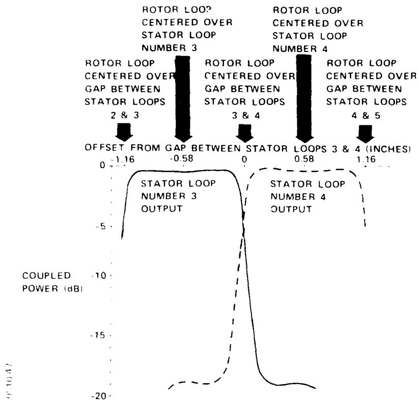
Figure 5-26. Measured loop-coupler power vs offset
