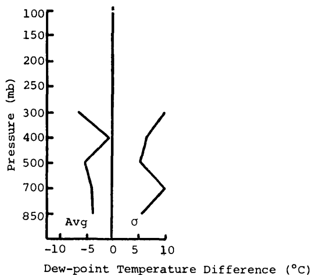
Fig. 28. Profiles of average and standard deviation of differences between satellite and rawinsonde dew-point temperatures (satellite minus rawinsonde) for the AVE-SESAME area.
