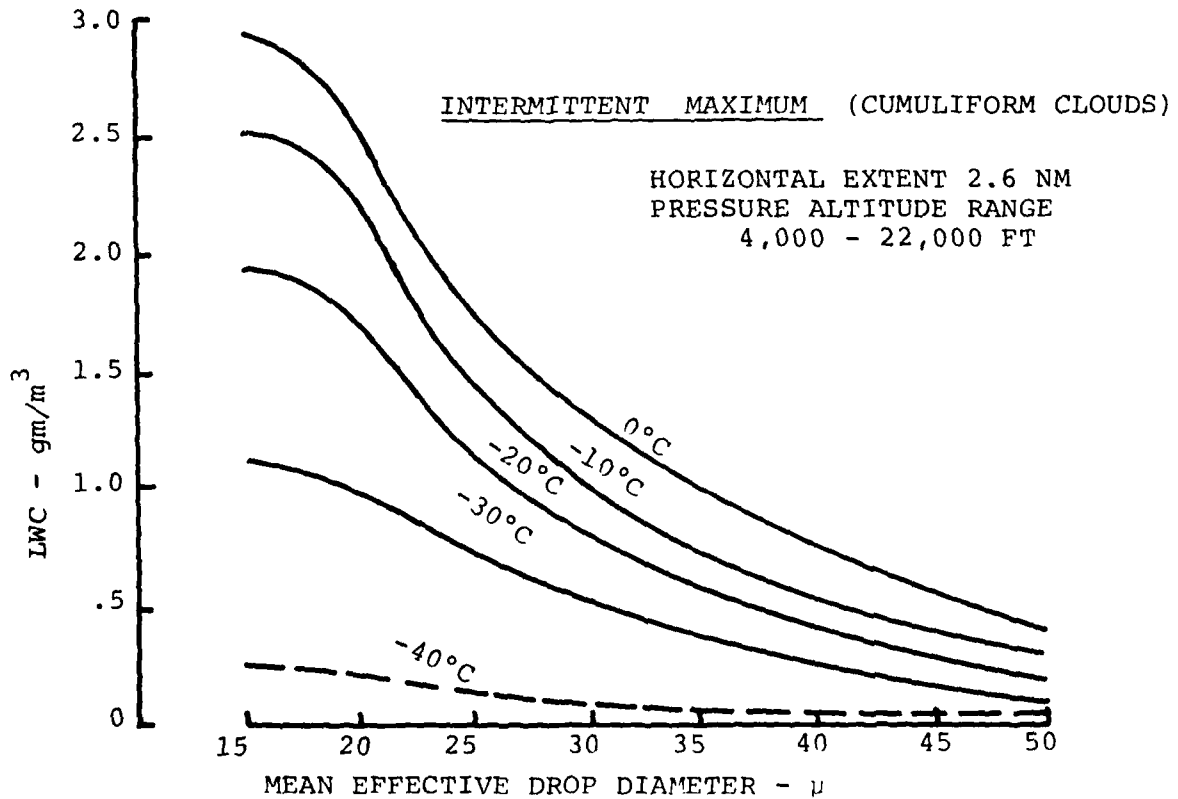
FIGURE 2-11. FAR PART 25 ICING LEVEL DEFINITIONS
