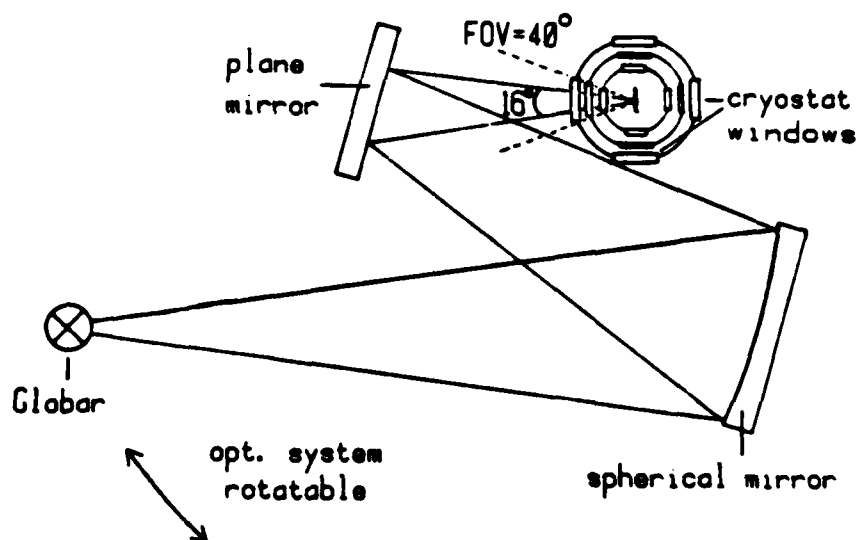
Fig. 5: Outline of the infrared optical system for illumination.
