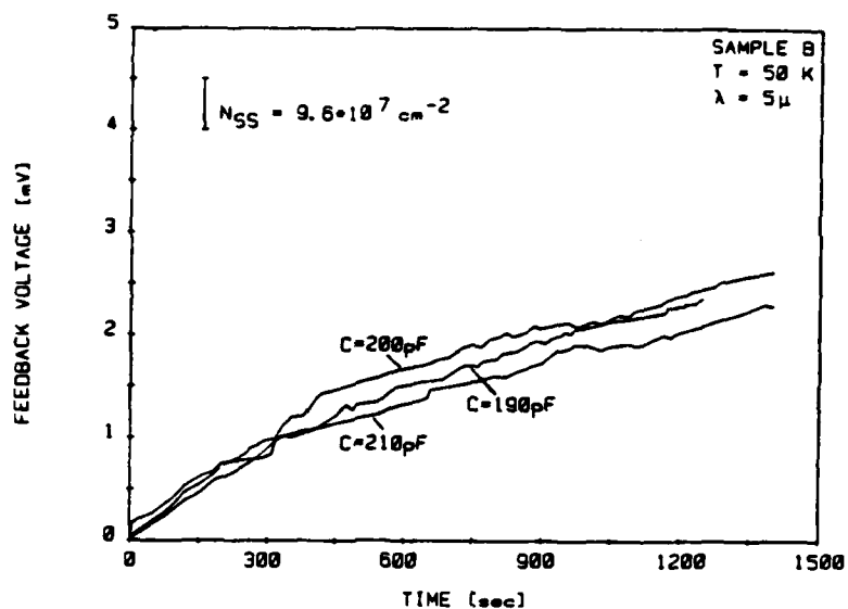
Fig. 15: Measured transients for photoexcitation in sample B. Parameter varied is the constant capacitance. Other data as shown in the insert.
