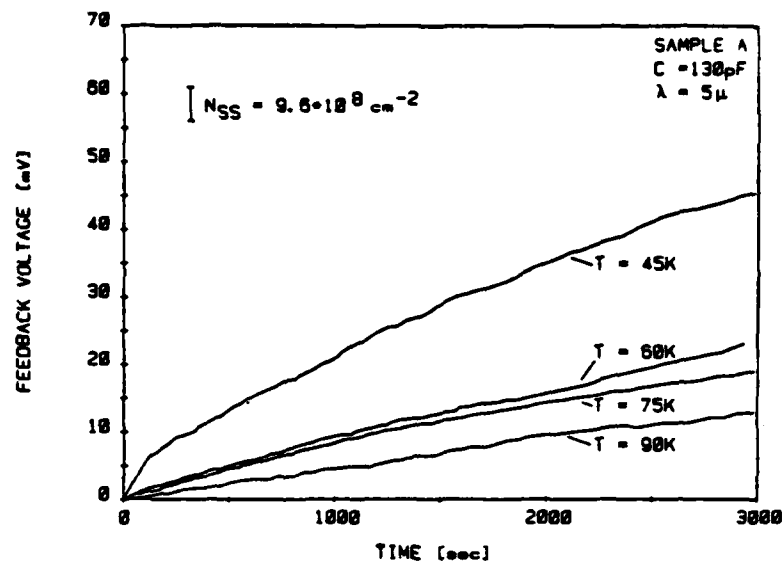
Fig. 13: Measured transients for photoexcitation in sample A with temperature as varied parameter. Other data as shown in insert.
