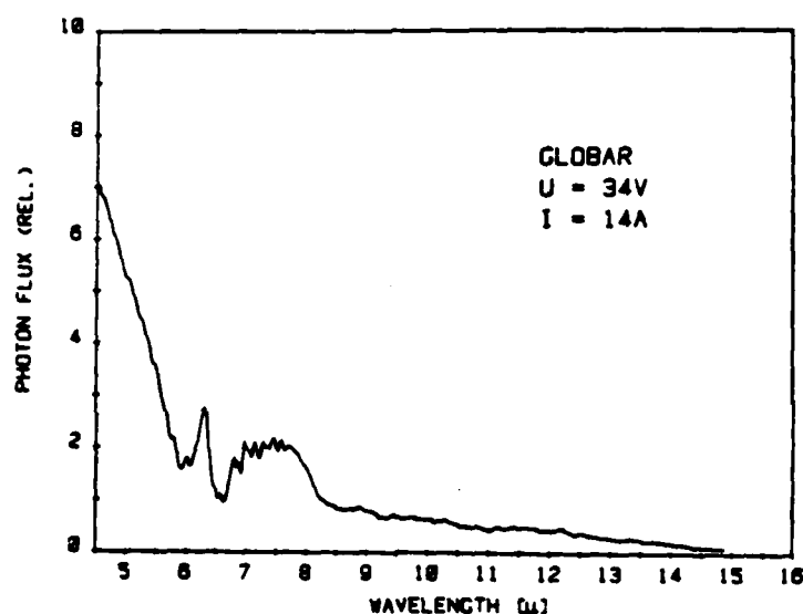
Fig. 6: Relative emission spectrum of globar IR-light source in wavelength region 5-15 \mu m.
