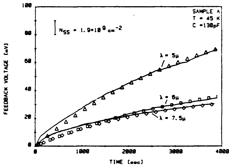
Fig. 16a: Computer fit for sample A at C = 130 \text{ pF} . The continuous lines are the measurements, the triangles, squares and rhombs the calculated fits.
