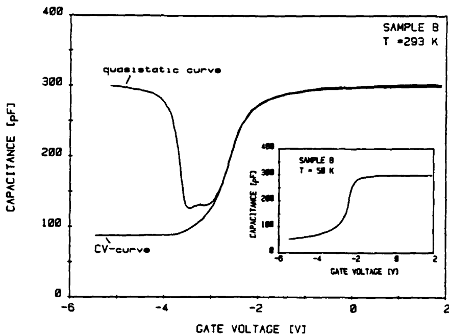
Fig. 10b: Result of CV-measurement of sample B at room temperature and at 50K in the insert.
