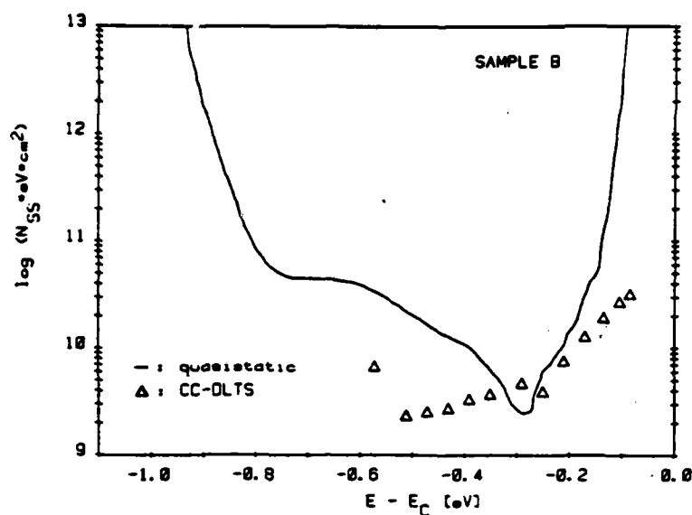
Fig. 11b: Interface state density as a function of energy for sample B as determined by quasistatic CV-technique (continuous line) and CC-DLTS (triangles)
