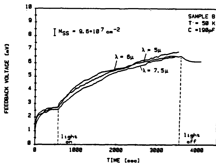
Fig. 14: Measured transients for photoexcitation in sample B. Parameter is the wavelength for excitation. Other data as shown in insert.
