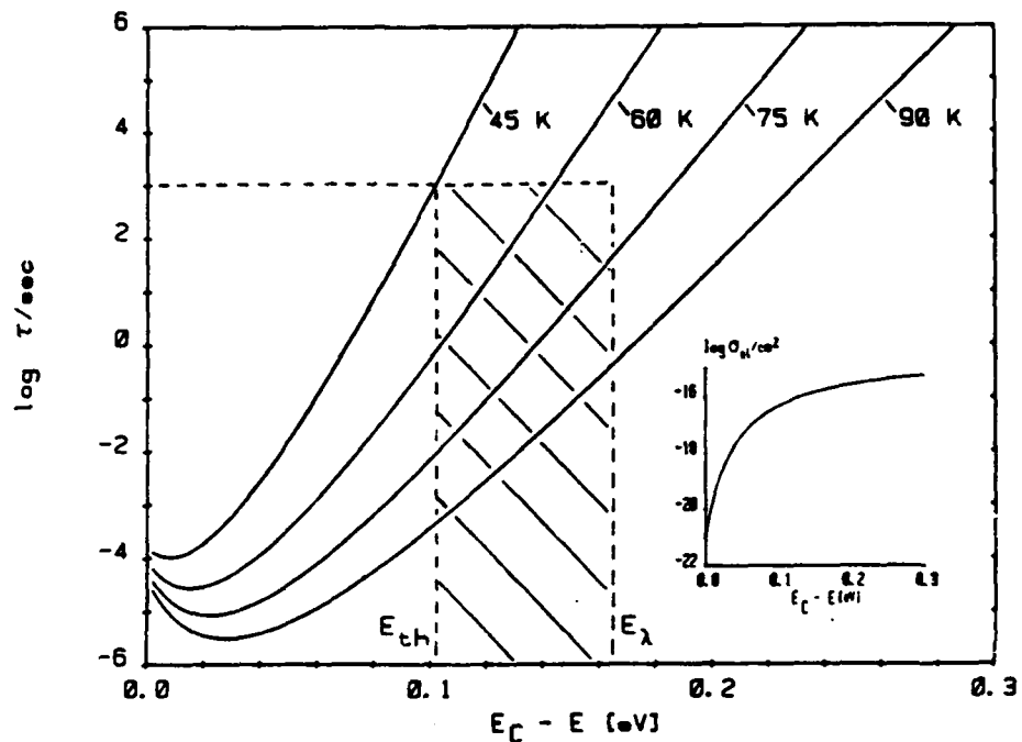
Fig. 3: Sketch of the time constant variation for thermal emission. Parameter is the sample temperature. Only states in the hatched energy region are available for the photoemission.
