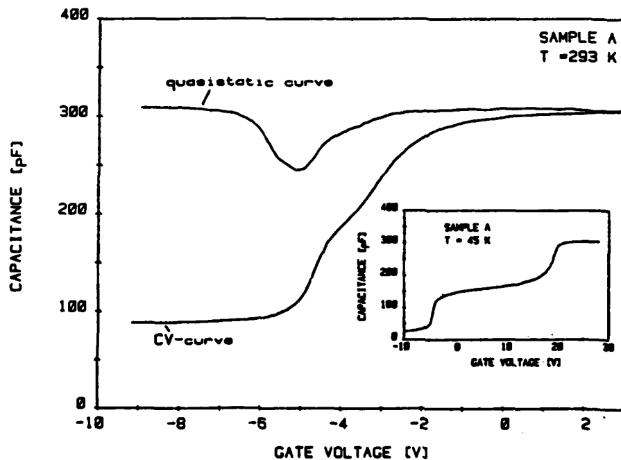
Fig. 10a: Result of CV-measurement of sample A at room temperature and at 45 K in the insert.
