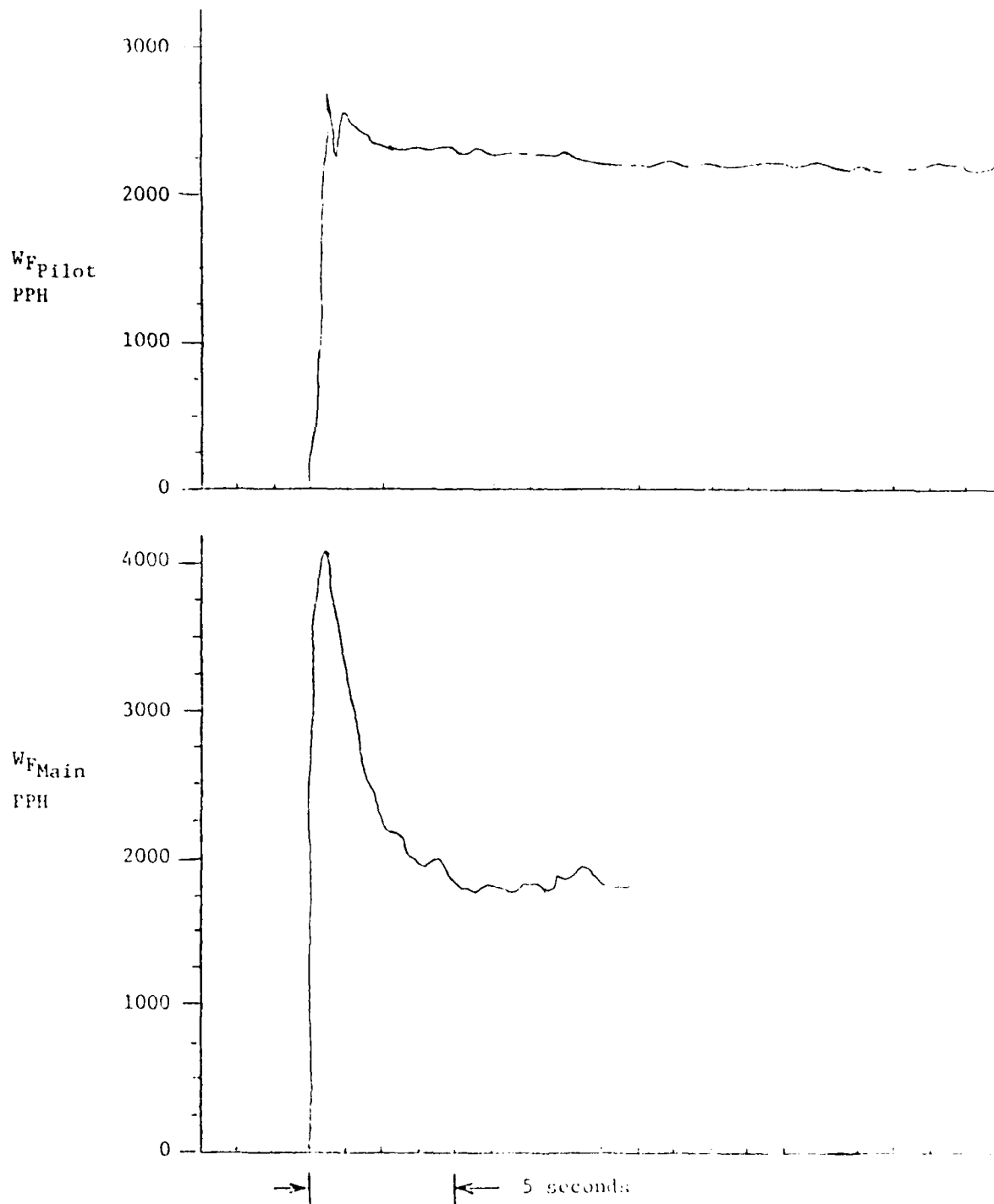
Figure 24. Stepped Responses of Pilot and Main Valves
