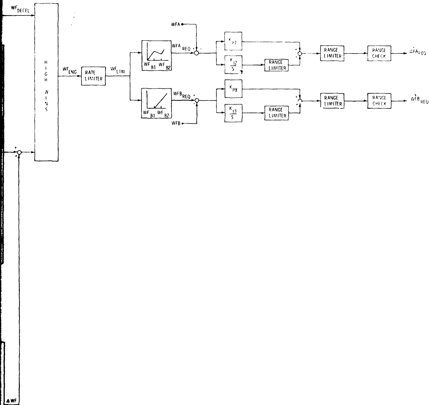
Figure 11. ATEGG Fuel Control Mode
