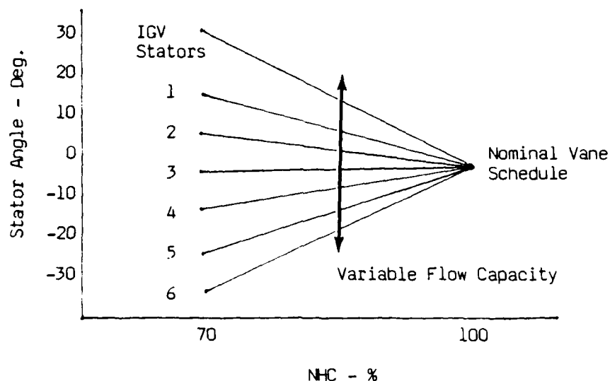
Figure 13. Compressor Surge Avoidance Relationship.
