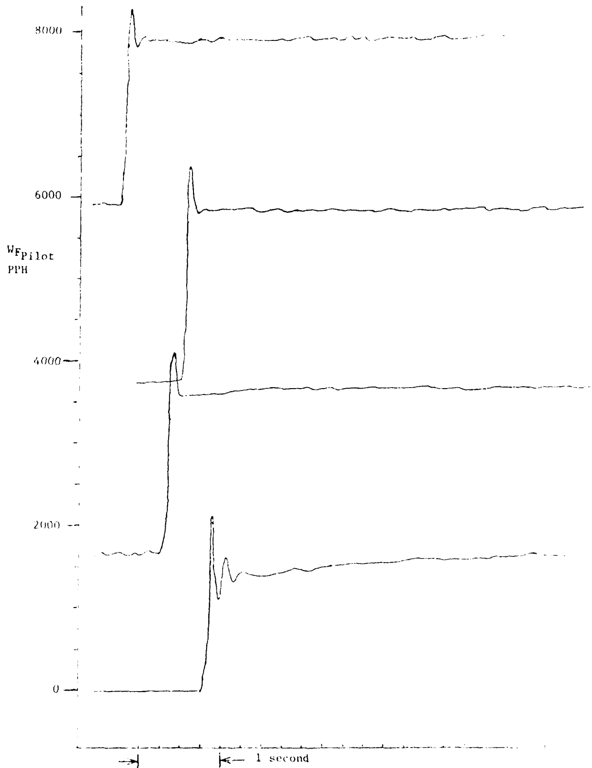
Figure 25. Pilot Valve Response - Final Configuration
