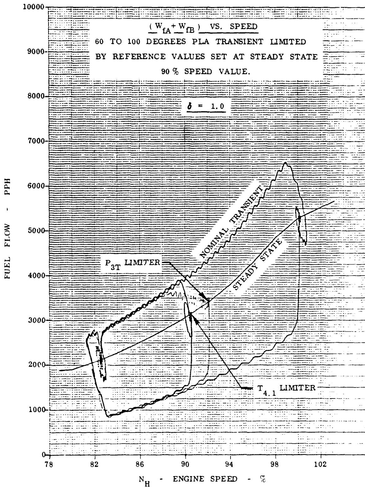
Figure 21. Parameter Limited Transients - Fixed RPR
