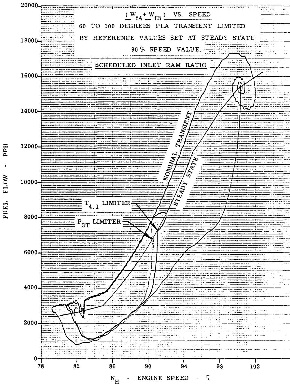
Figure 20. Parameter Limited Transients - Scheduled RPR
