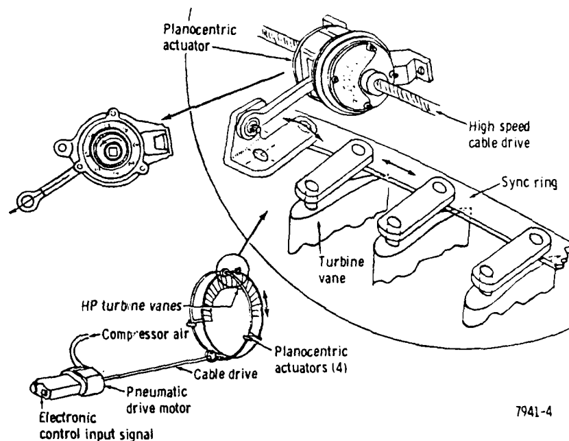
Figure 4. HP turbine vane actuation system.
