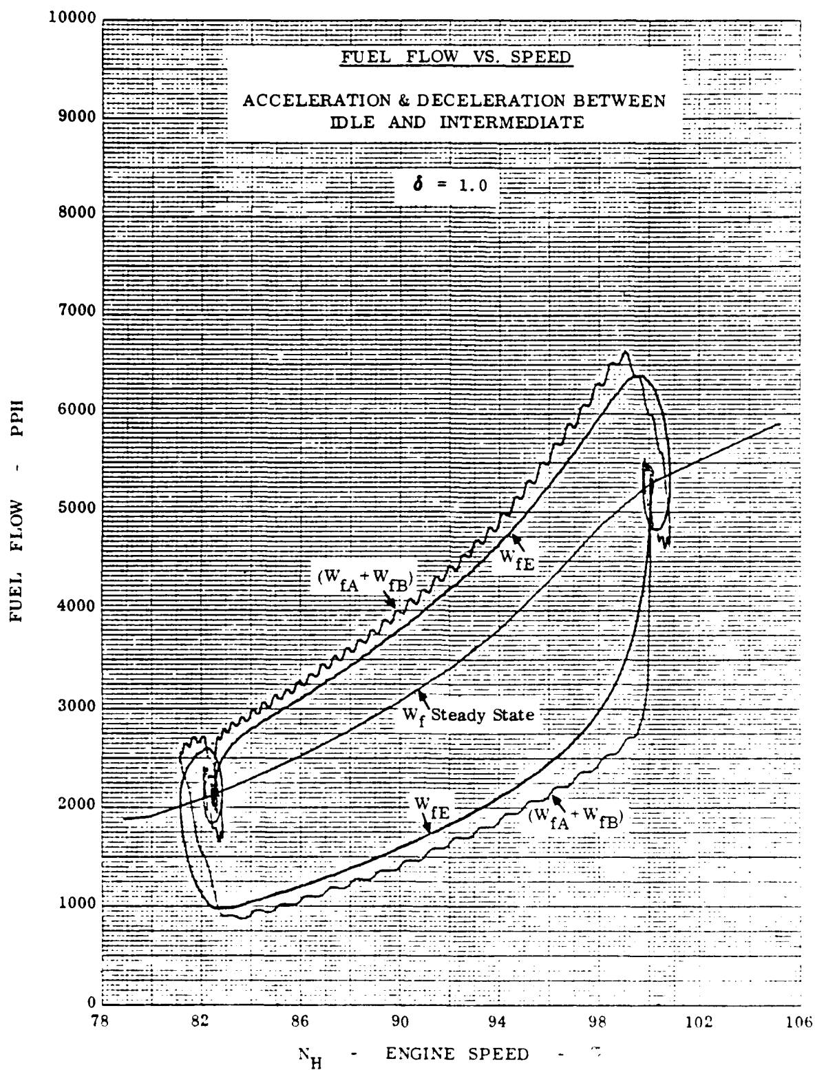
Figure 19. Transients between Idle and Intermediate - Fixed RPR
