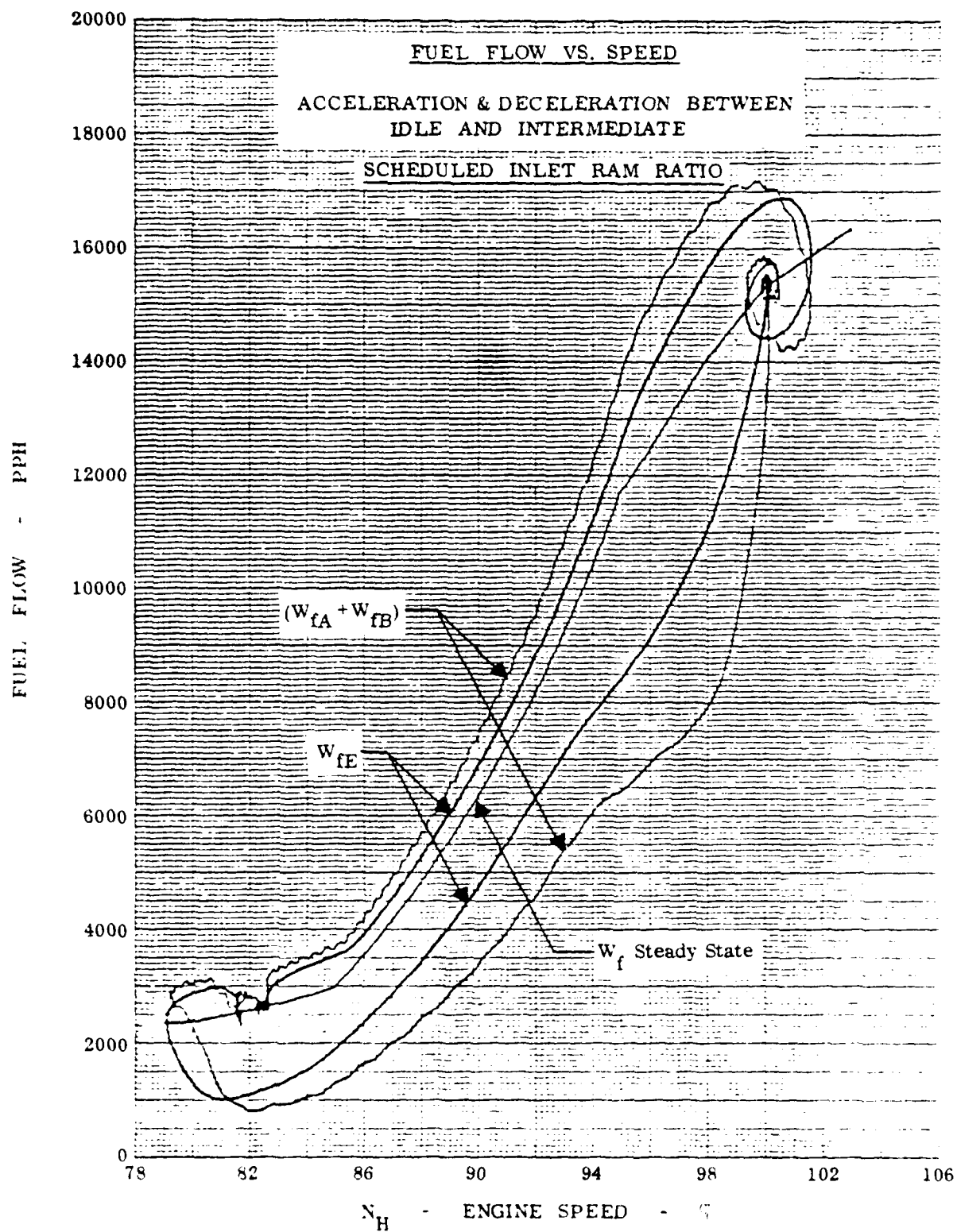
Figure 18. Transients between Idle and Intermediate - Scheduled RPR
