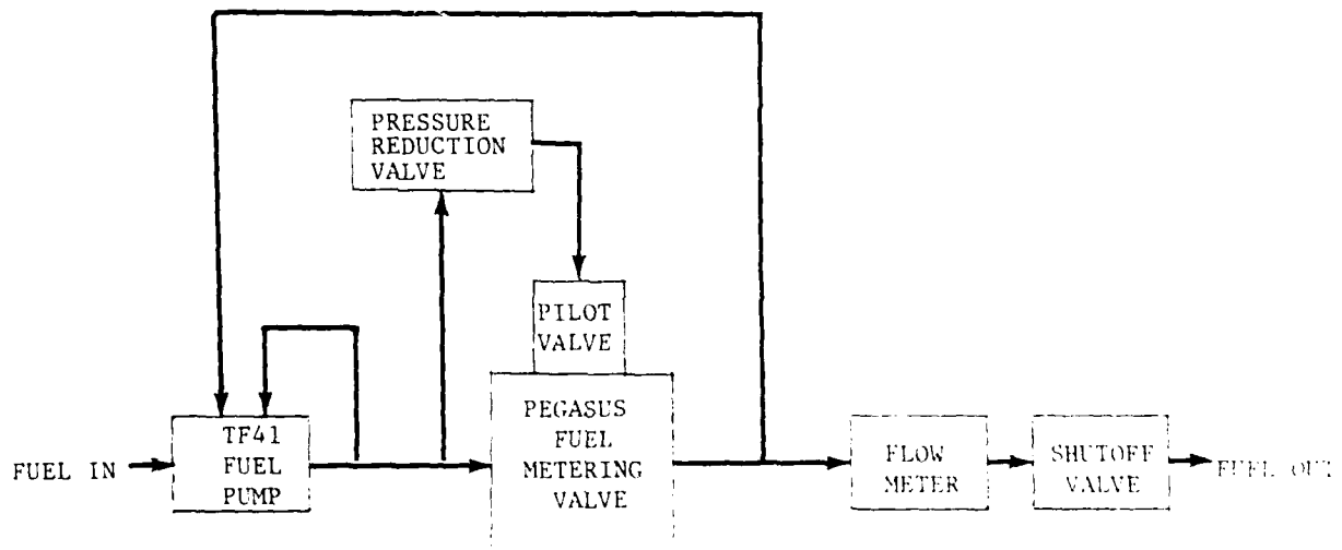
Figure 3. GMA200 Fuel System
