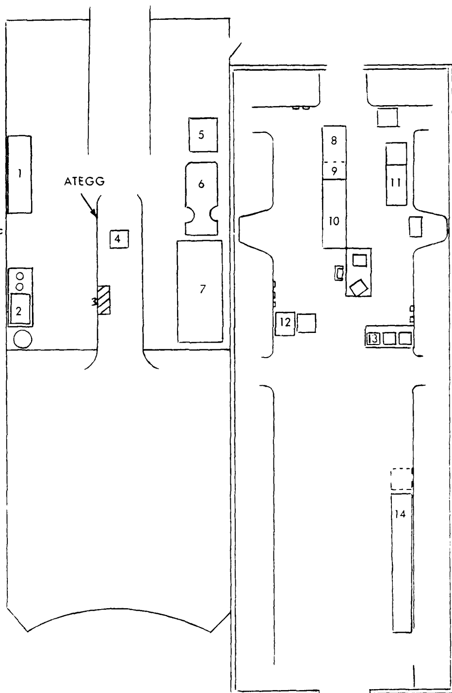
Figure 29. Test Cell 882 & Control Room Layout
