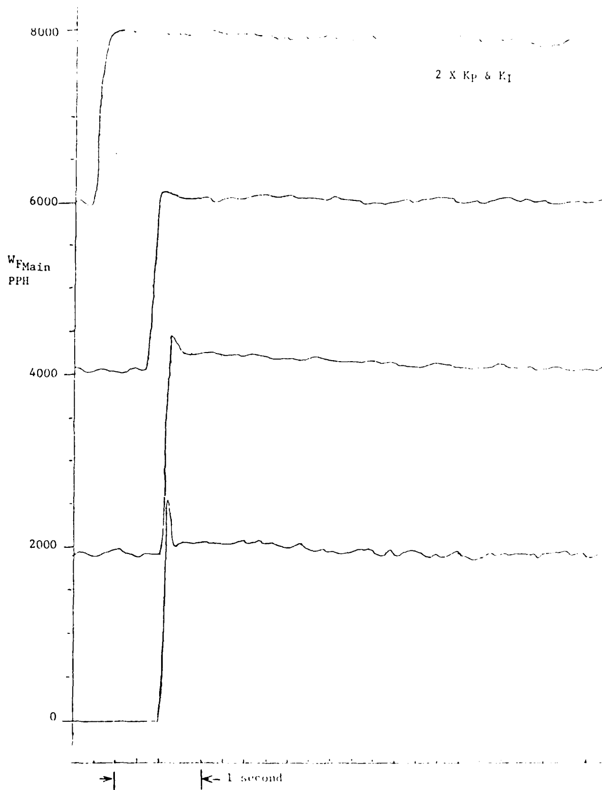
Figure 26. Main Valve Response - Final Configuration
