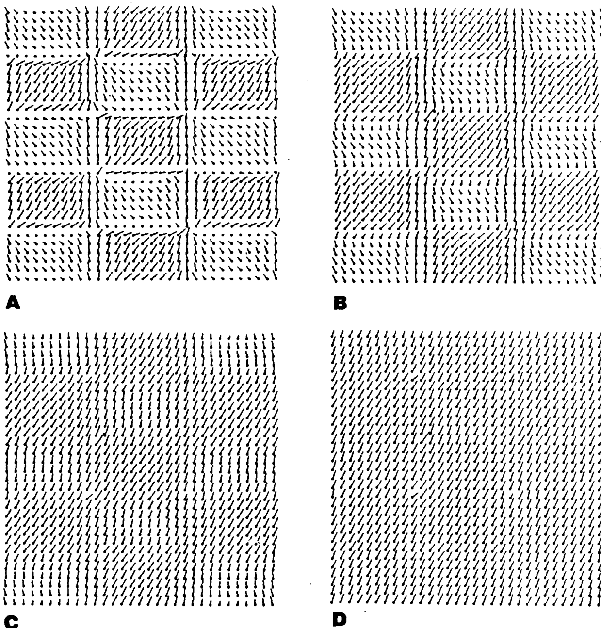
Figure 6. Flow pattern computed for simple translation of a brightness pattern. The estimates after 1, 4, 16, and 64 iterations are shown. The velocity is 0.5 picture cells in the x direction and 1.0 picture cells in the y direction per time interval. Two images are used as input, depicting the situation at two times separated by one time interval.
