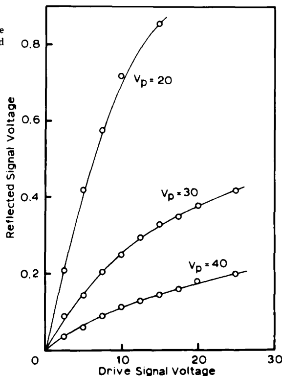
Fig. 4. Reflection cell output voltage as a function of square-wave signal drive voltage with pedestal voltage as a parameter. Liquid crystal was a 0.5% cholesteric with a thickness of 1/2 mil.
