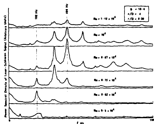
Fig. 14 Laser-schlieren spectra, equivalence ratio fixed Re varied.
