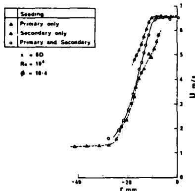
Fig. 8 Mean velocities measured in Jet Flame 1 with three types of LDA seeding.
