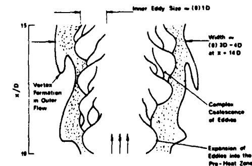
Fig. 3c Structure of Jet Flame I, 10 < x/D < 15
