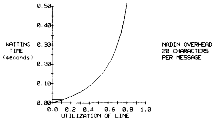
FIGURE 4.7: DELAYS ON CONCENTRATOR TO SWITCH LINE (4.8 Kb/s)
