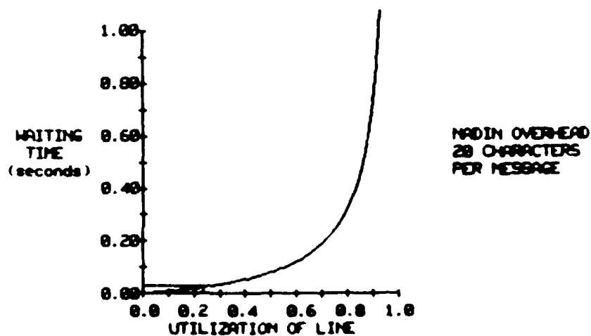
FIGURE 4.5: DELAYS ON SWITCH TO CONCENTRATOR LINE (4.6 KB/s)
