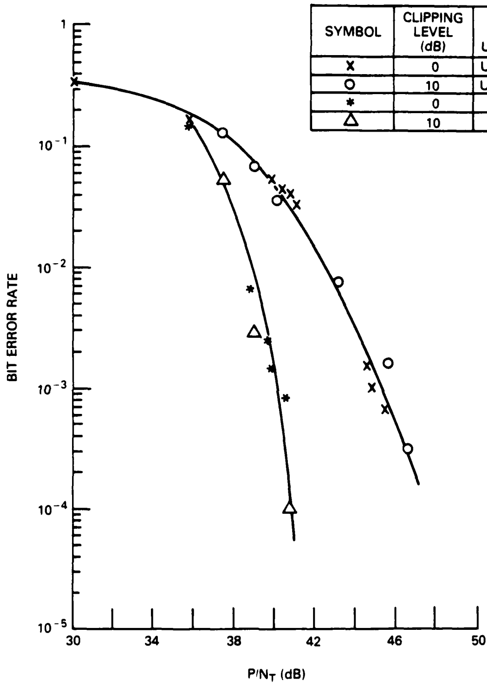
Fig. 6 - Bit error rate on coded and uncoded voice versus P/N_T
