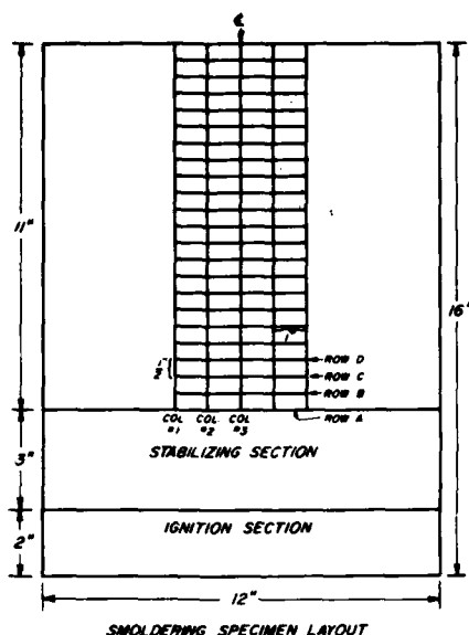
Figure 1.—Specimen with scribed grid for smoldering test.
