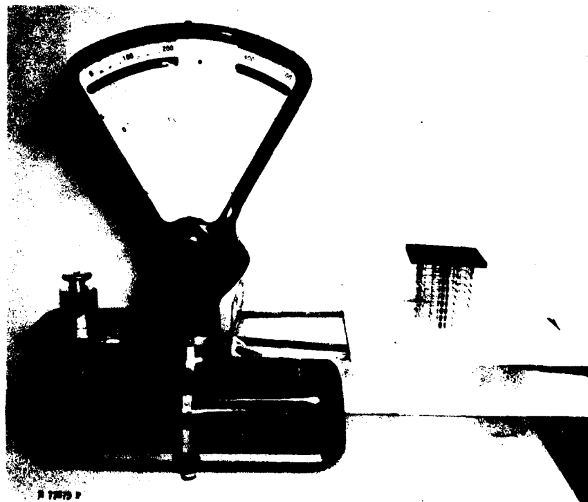
Figure B-2.—Apparatus for testing glow performance of insulation boards, showing test specimen in position. (M 77875 F)
