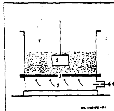
Fig.1. Diagram of a device for generating coatings by the fluidization method. 1-upper part of the bath; 2-lower part of the bath; 3-porous partition; 4-inlet of pressurized air; 5-object being coated; 6-whirling powder being liquefied (fluidization bed).
