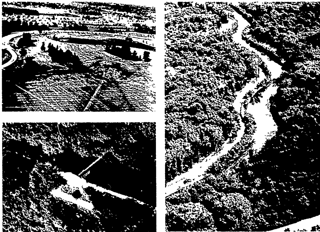
Figure 30. Portions of the Cook County, Illinois Forest Preserve District along the Des Plaines River. Note the remarkable similarity of the land forms, woodlands and river to the study area in Texas.
