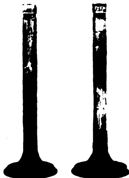
FIGURE G-12 HATZ INTAKE AND EXHAUST VALVES AFTER THE PERFORMANCE TEST, VIEW 1
