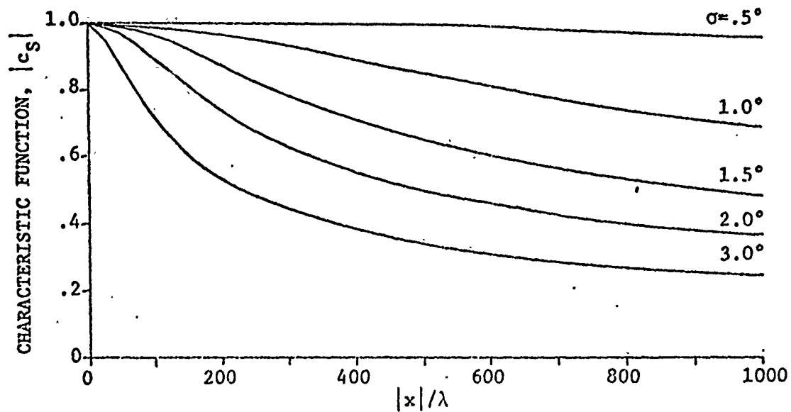
Fig. 5.6 Characteristic function for spatial multipath interference.
