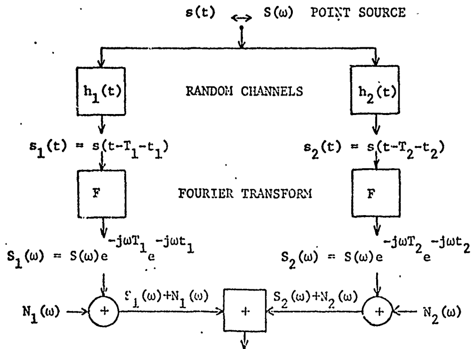
Fig. 2.7 Signal processing for random channels.
