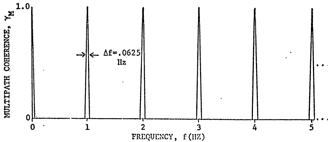
Fig. 5.14 Auto-coherence due to frequency selective multipath interference.
