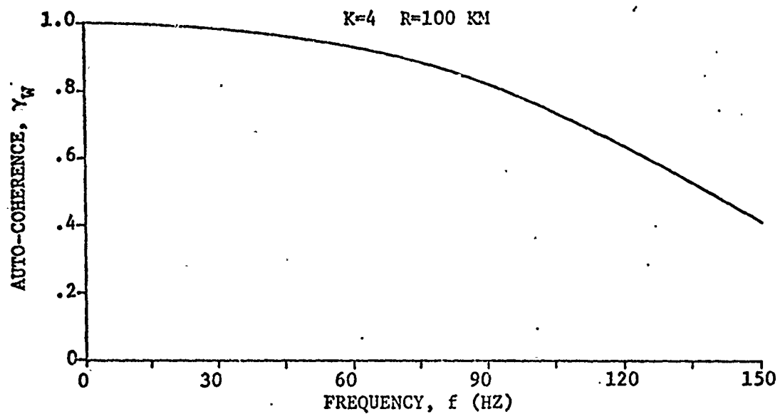
Fig. 5.5 Frequency variation of internal wave auto-coherence.
