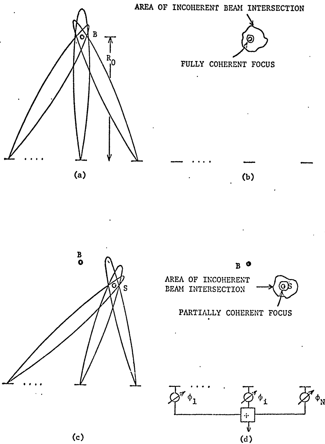
Fig. 6.1 VLA beamforming and scanning.
