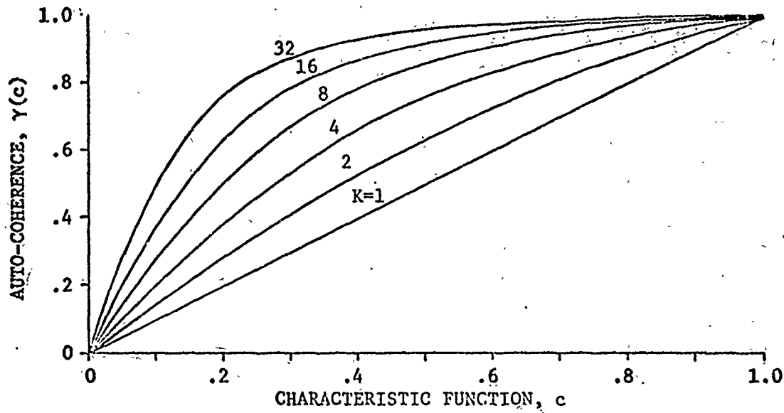
Fig. 5.15 General form of auto-coherence.
