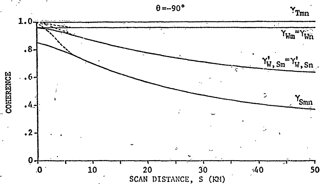
Fig. 5.18 Comparison of auto-coherences-- \theta = -90^\circ .
