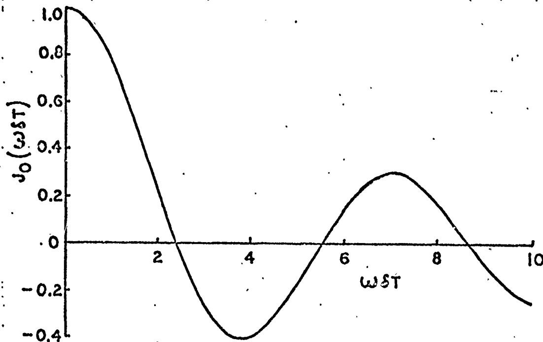
Fig. 5.11 Coherence due to internal tides.
