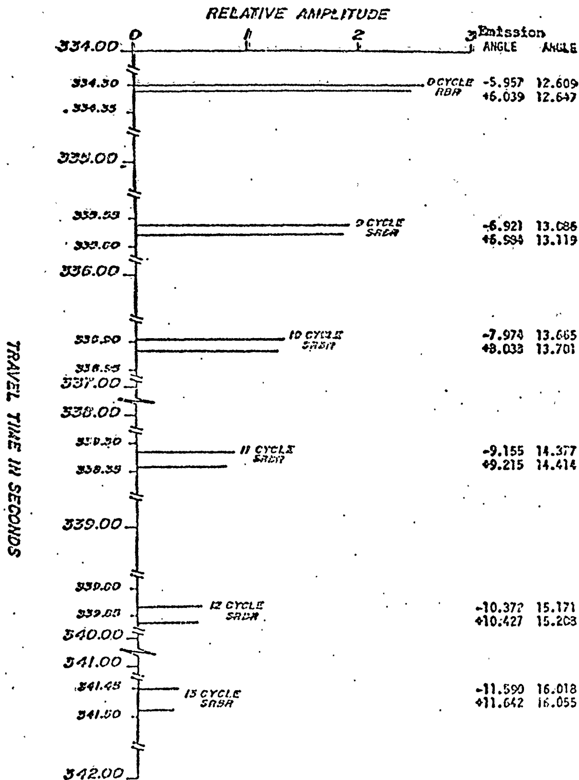
Fig. 2.3 Ray travel times, pressure amplitudes, and arrival angles (from reference 9, Chapter 3).
