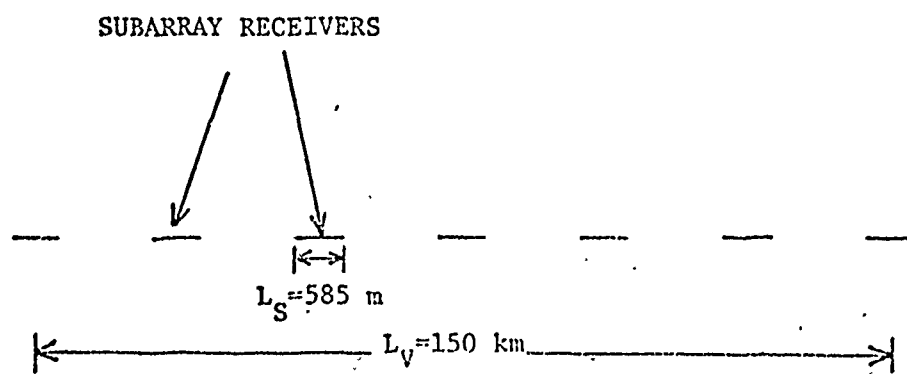
Fig. 6.3 VLA configuration for design example.
