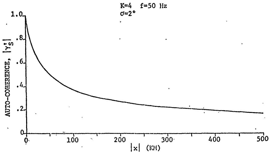
Fig. 5.8 Range variation of auto-coherence due to spatial multipath interference.
