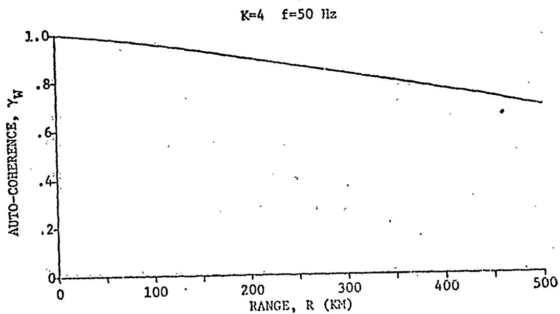
Fig. 5.4 Range variation of internal wave auto-coherence.
