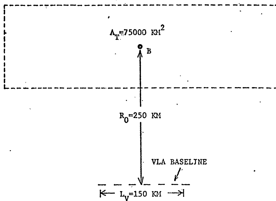
Fig. 6.4 VLA coverage area for design example.
