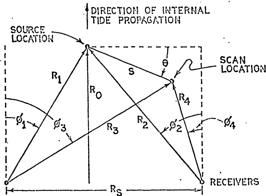
Fig. 5.10 Source-receiver configuration for internal tide fluctuations.
