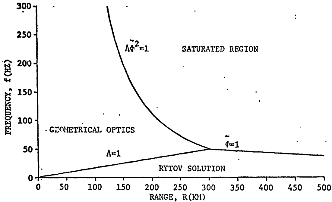
Fig. 2.6 \Lambda - \phi diagram for internal waves.
