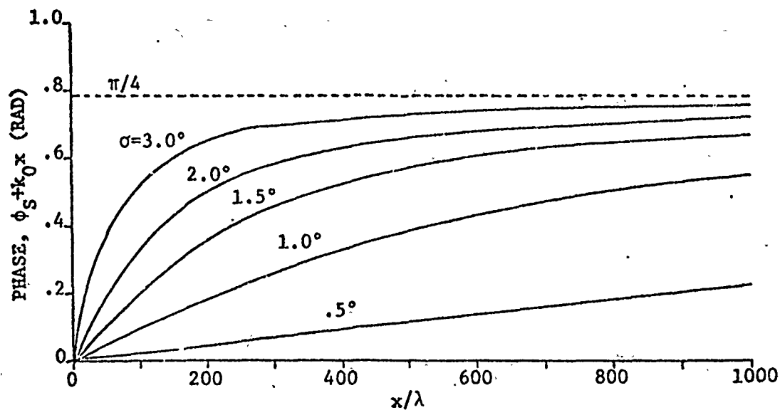
Fig. 5.7 Average phase variation due to spatial multipath interference.
