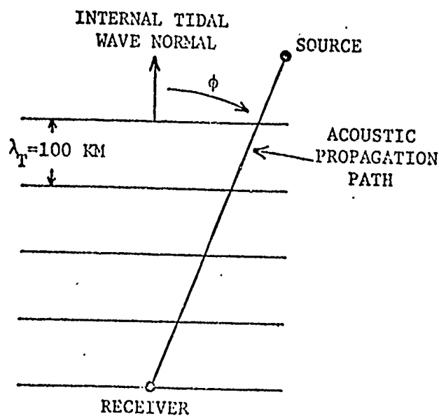
Fig. 3.3 Acoustic propagation geometry for internal tide fluctuations.
