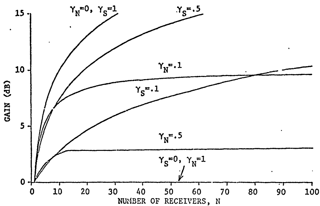
Fig. 2.10 Comparison of conventional array gain with VLA gain.
