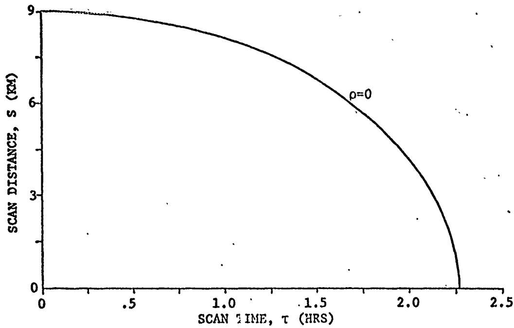
Fig. 5.1 Scan distance and scan time for uncorrelated internal wave fluctuations.
