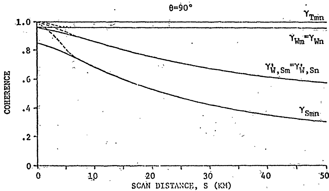
Fig. 5.16 Comparison of auto-coherences-- \theta = 90^\circ .
