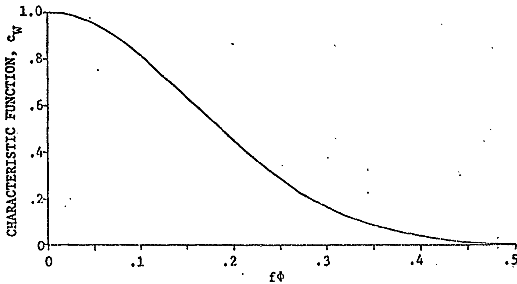
Fig. 5.2 Characteristic function for internal wave fluctuations.
