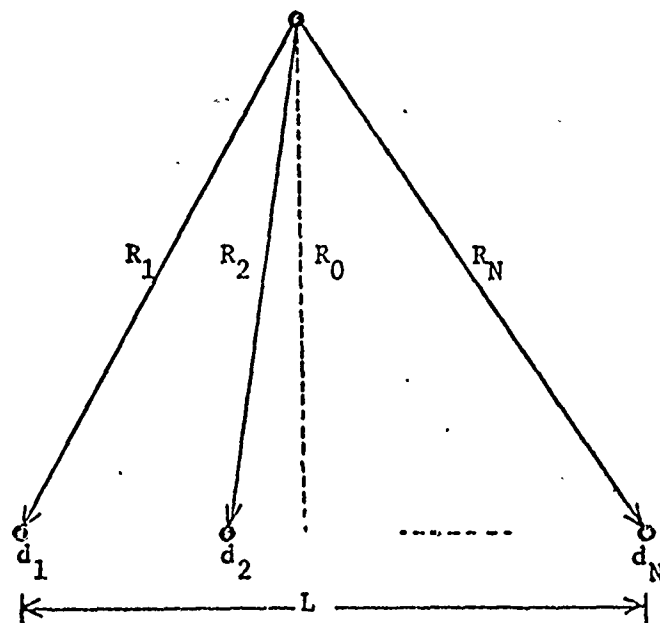
Fig. 2.9 Configuration of VLA.
