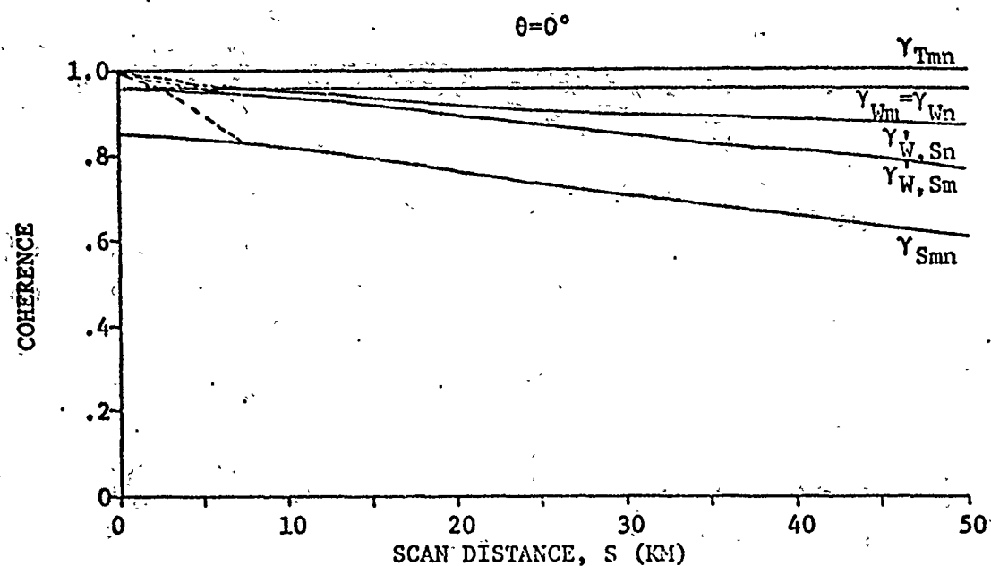
Fig. 5.17 Comparison of auto-coherences-- \theta = 0^\circ .
