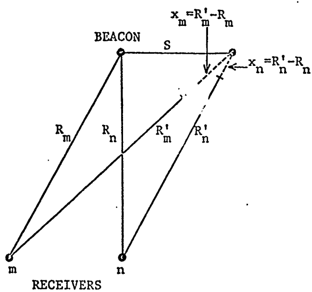
Fig. 4.3 Scanning geometry.
