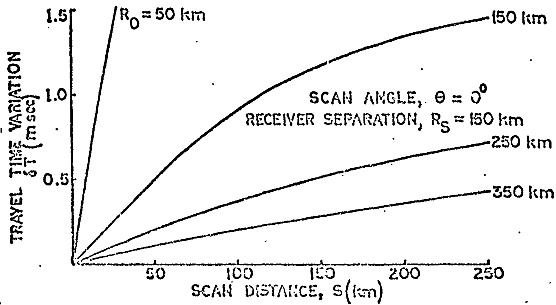
Fig. 5.12 Travel time fluctuation due to 4m amplitude internal tide.
