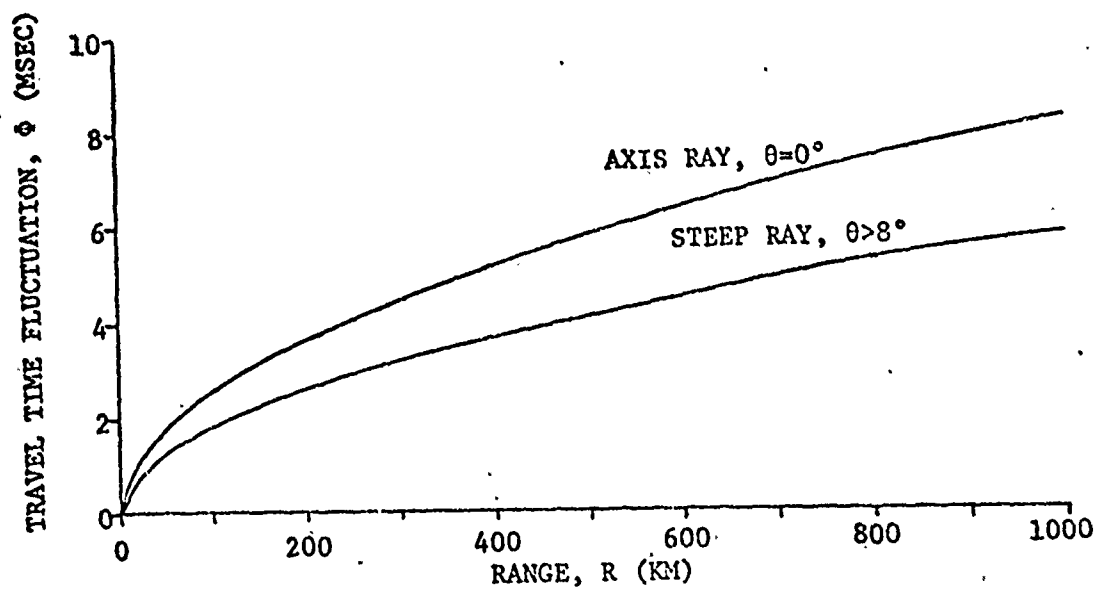
Fig. 5.3 RMS travel time fluctuation due to internal waves.
