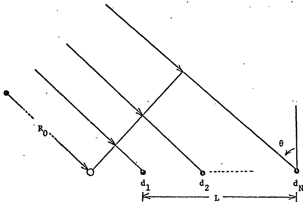
Fig. 2.8 Configuration of conventional array.
