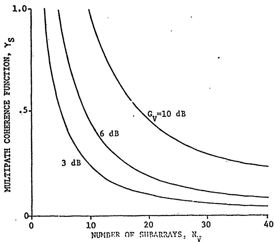
Fig. 6.2 Required value of MCF for specified VLA gain.
