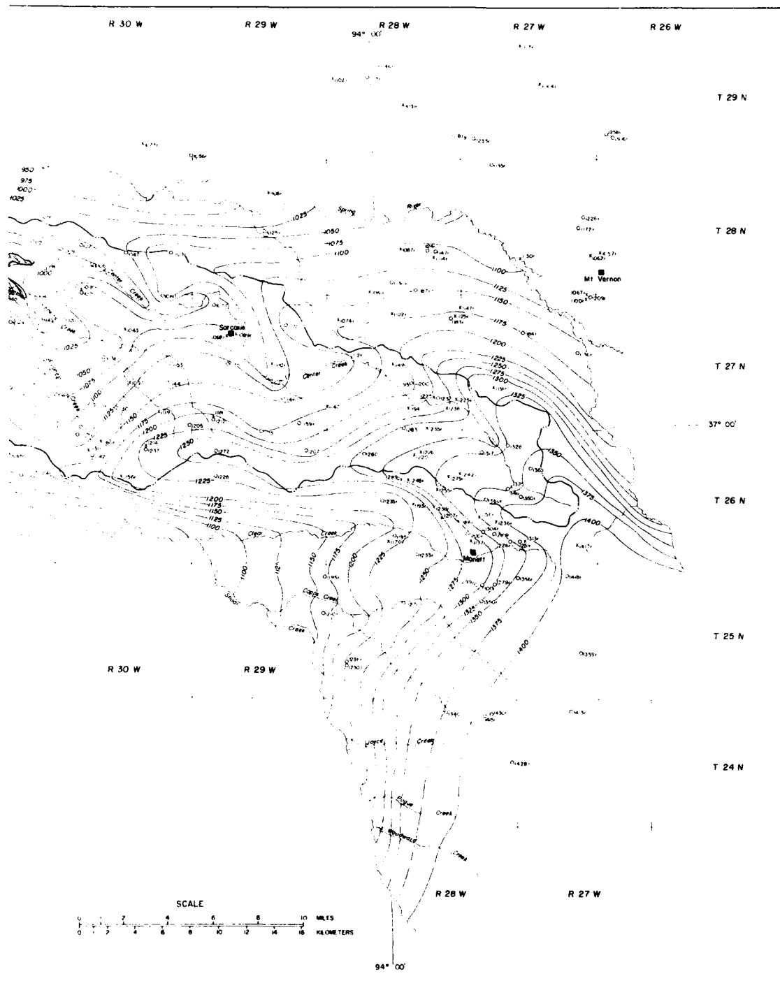
contiguous parts of Spring River and Shoal Creek basins, Missouri, 1978. (Contour interval, 25 ft.)
