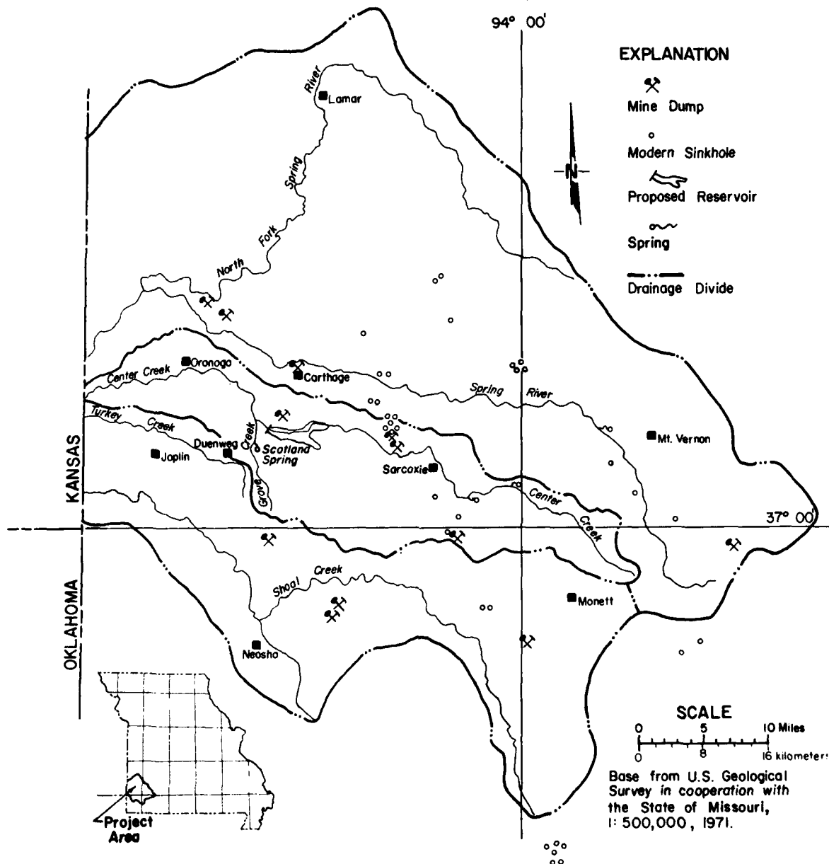
Figure 1.-- Map of Center Creek basin showing location of proposed reservoir, mine dumps, and sinkholes.
