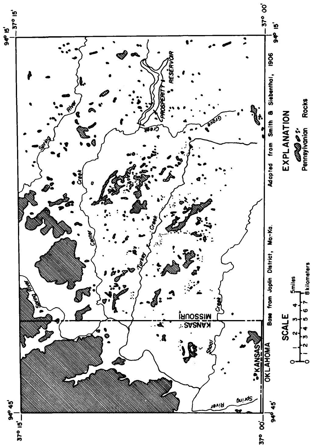
Figure 5.-- Distribution of Pennsylvanian rocks in the Joplin area
