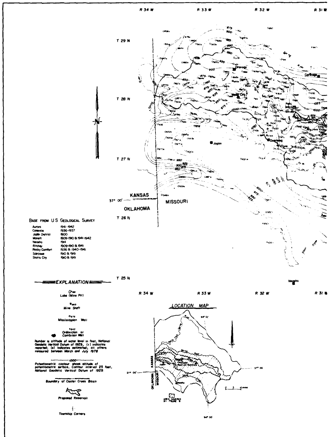
Figure 9.-- Potentiometric map of Mississippian limestone aquifer in Center Creek basin and area.
