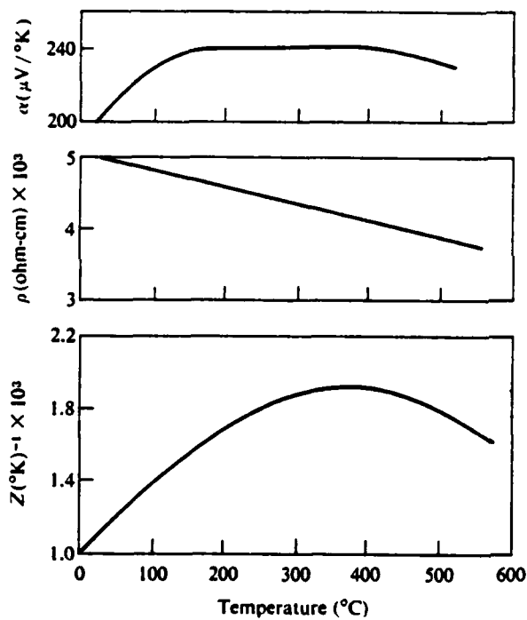
The Seebeck coefficient, electrical resistivity, and figure of merit of a p -type alloy: AgSbTe 3 .
