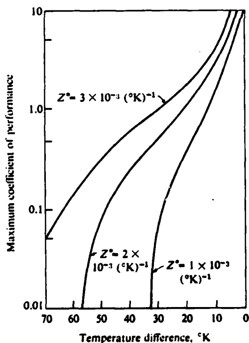
The maximum coefficient of performance that can be achieved with a given temperature difference and a specified figure of merit for the couple. The hot shoe temperature is assumed to be 300^{\circ}K .
