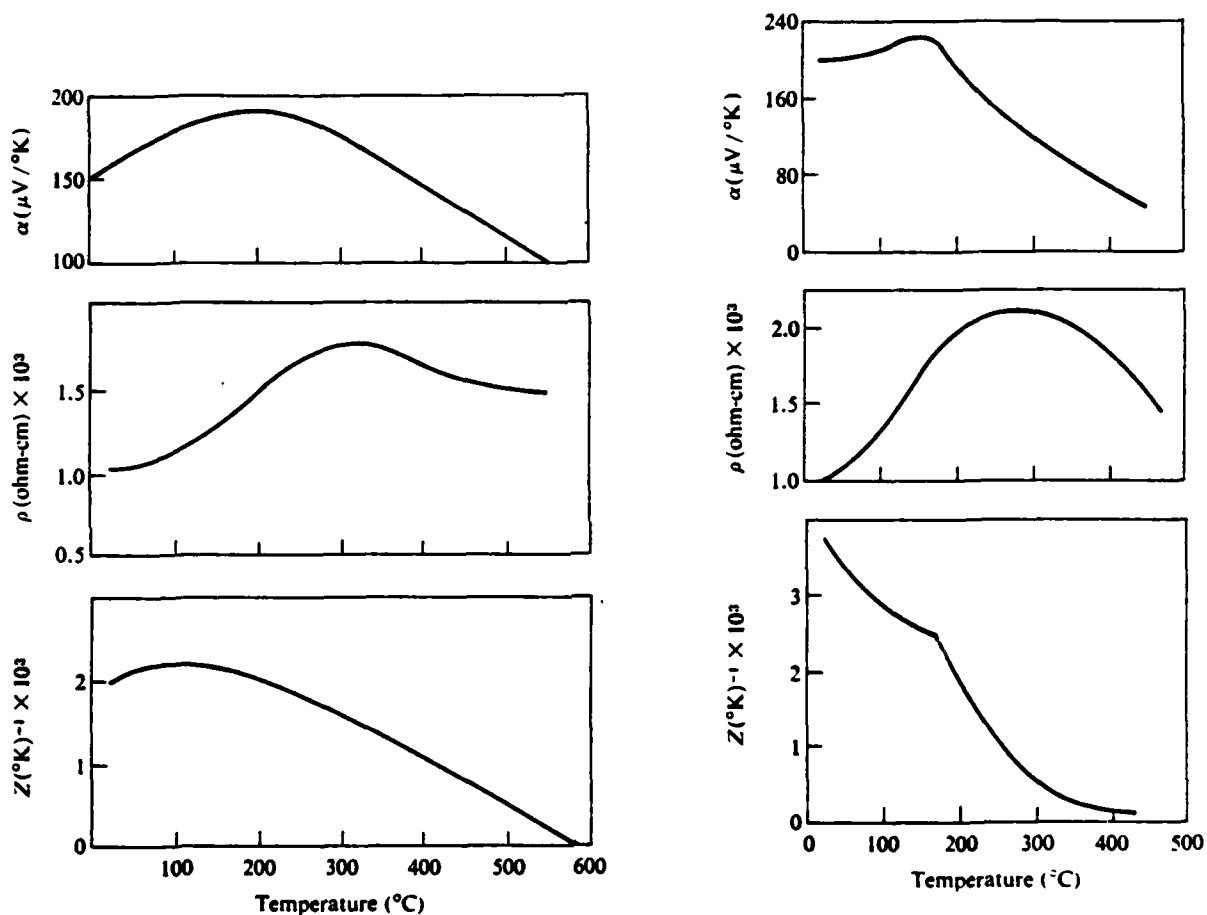
The Seebeck coefficient, electrical resistivity, and figure of merit of a p -type alloy: 25% Bi 2 Te 3 , 75% Sb 2 Te 3 (1.75% Se).
