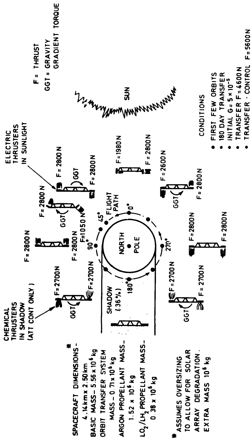
Fig 49 Thrusting strategy for rectangular section of 10GW SPS during spiral orbit raising (Boeing - Ref 43)
