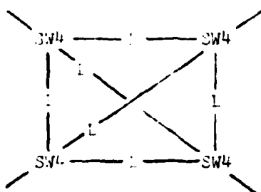
A) Four node DDC "star" network built from completely utilized SW4 HIPs.
