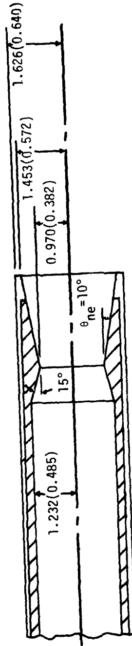
(b) 10° Conical Nozzle, the C1 Nozzle.
