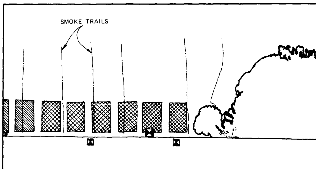
Figure 6. Fireball perturbation observed on 5-ton TNT block-built hemispherical charge. (Sketch made by the author from a photograph in Reference 15; original could not be located.)
