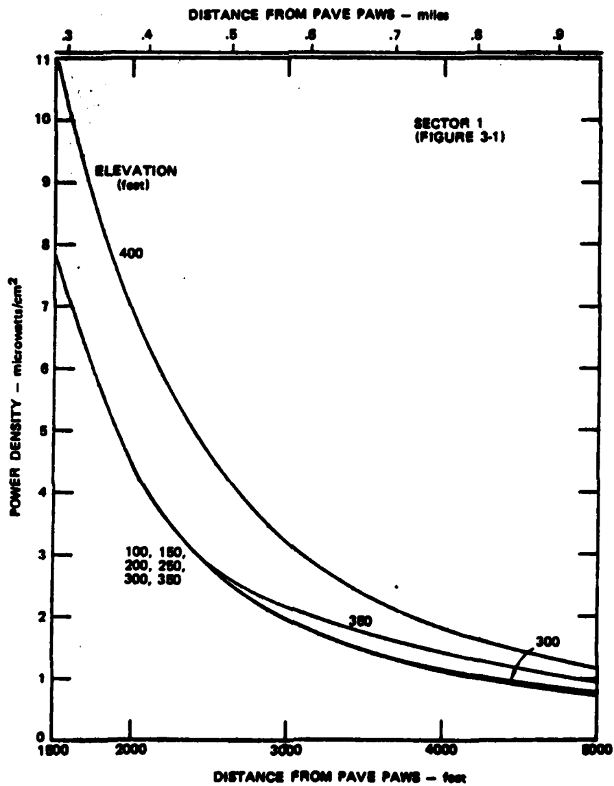
FIGURE 3-3. CALCULATED PAVE PAWS EMR POWER DENSITY FOR SECTOR 1, 1,500-8,000 FT RANGE
